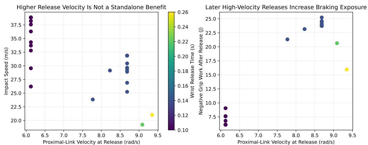
Figure 6.4: Release-state proximal velocity against impact speed and negative grip work for every valid-impact trajectory. Color denotes release time, exposing the timing confound.
