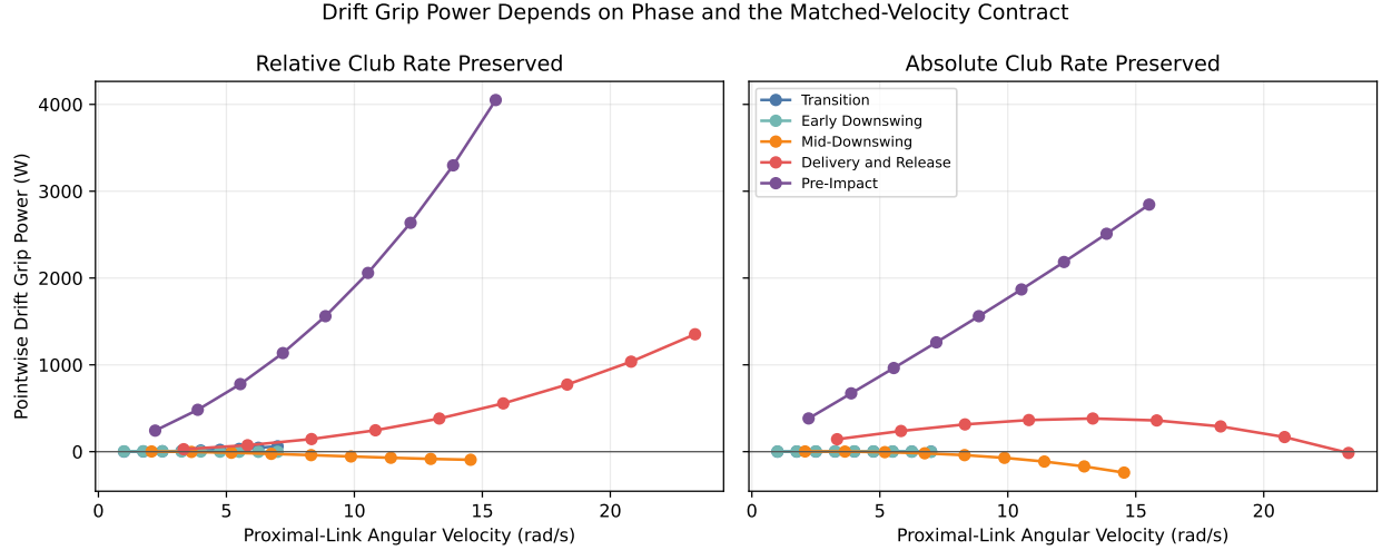
Figure 6.1: Drift grip power across proximal angular-velocity sweeps. Each panel states the velocity-matching rule; the large late-swing benefit is not invariant to that rule.
