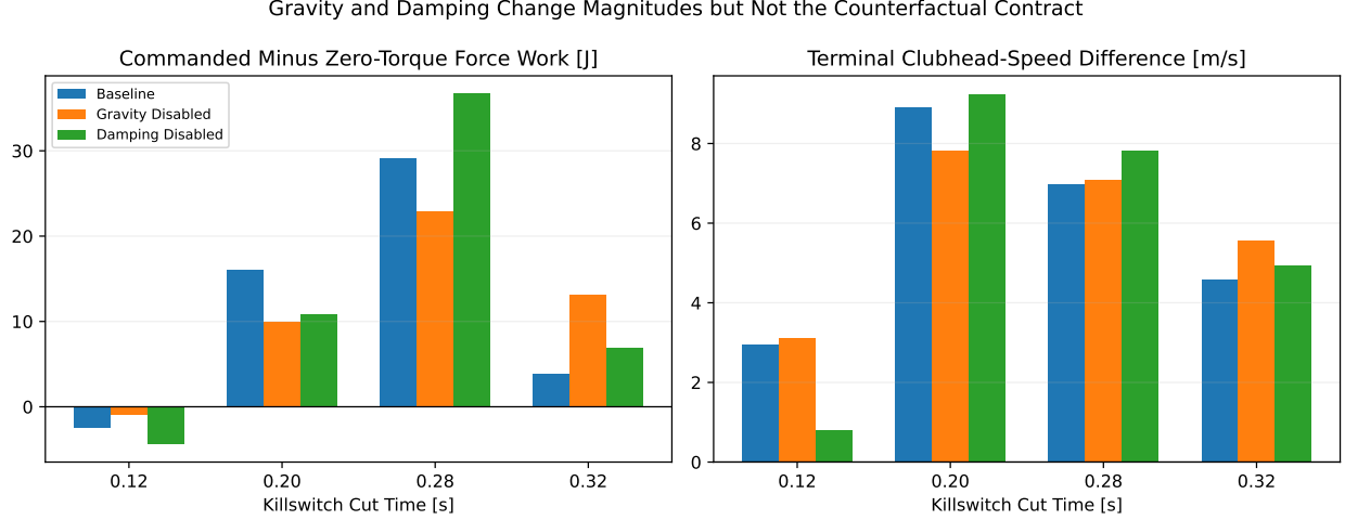
Figure 7.4: Gravity and Damping Ablations of the Killswitch Comparison
