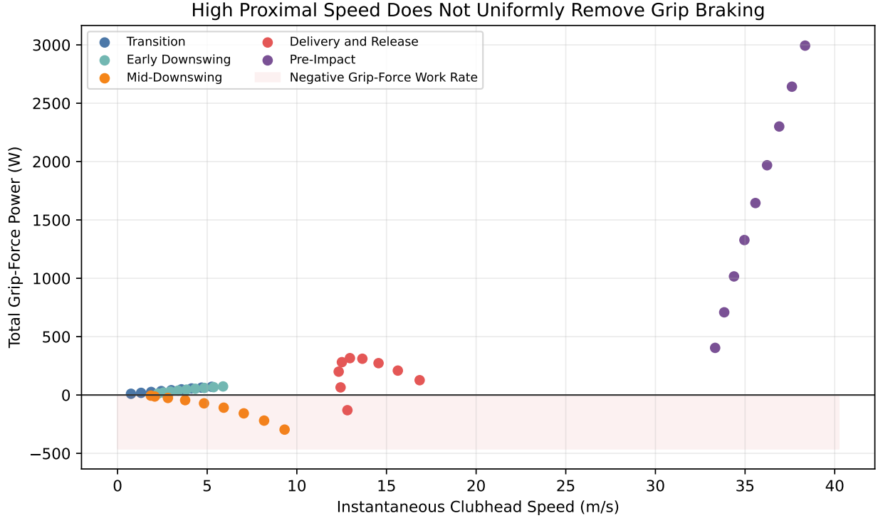
Figure 6.2: Negative grip power across phase and velocity-matching rule. Shading marks states in which the grip reaction removes modeled mechanical energy from the club at that instant.
