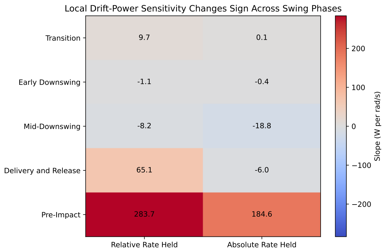
Figure 6.3: Signed slope of drift grip power with proximal angular velocity. Positive cells indicate that faster proximal motion increases drift-mediated grip power within the declared local sweep.
