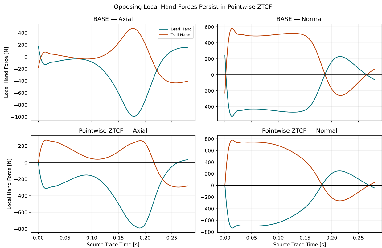
Figure 7.5: Opposing Local Hand Forces Persist in Pointwise ZTCF
