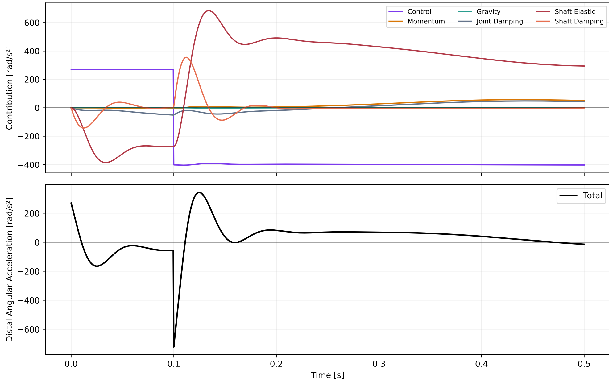
Momentum, Gravity, Damping, Control, and Shaft Terms Sum Exactly
