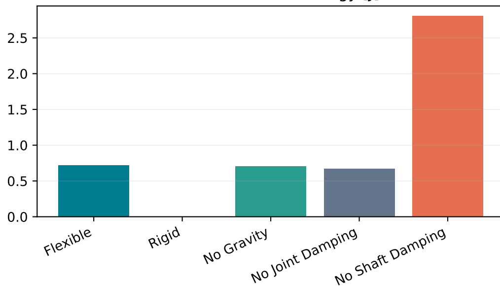
Peak Shaft Strain Energy [J]
