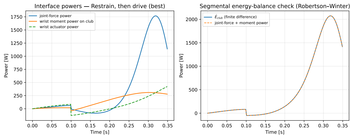
Figure 11.7: Left: wrist-interface powers for the best restrain-then-drive swing. Right: segmental energy-balance check — club mechanical-energy rate versus the sum of interface powers.
