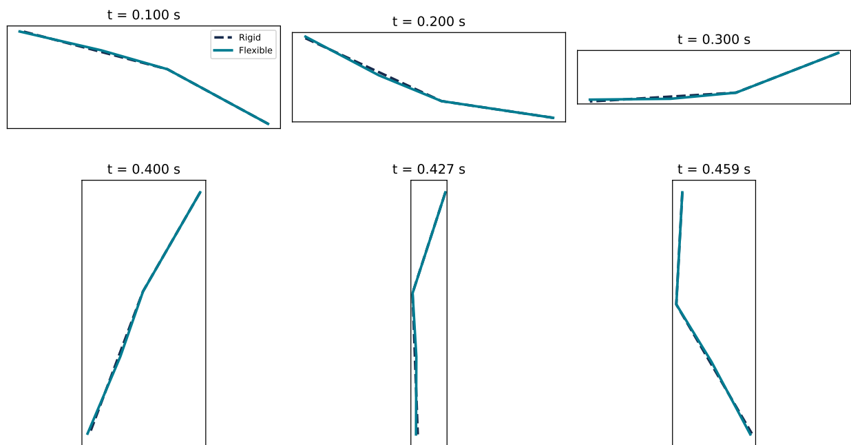
Figure 10.5: Flexible and Rigid Centerlines Separate Near Delivery
