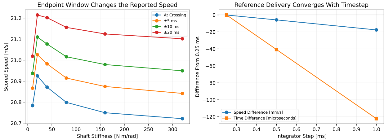
Figure 10.8: Impact Definition and Numerical Resolution
