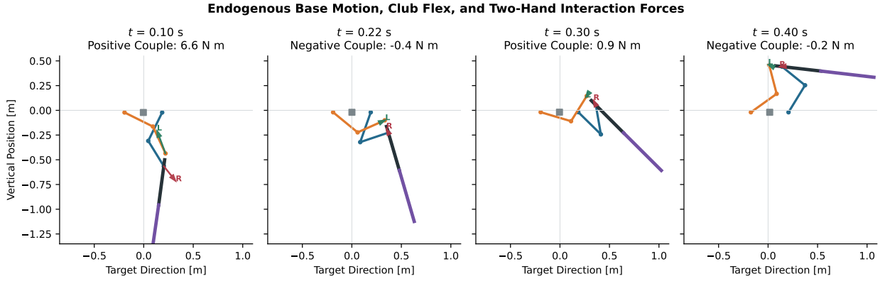
Figure 11.1: Endogenous Base Motion, Club Flex, and Two-Hand Interaction Forces
