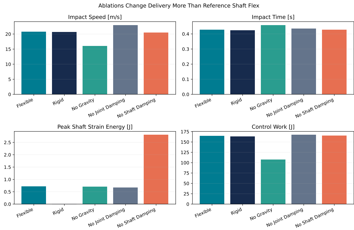
Figure 10.6: Ablations Change Delivery More Than Reference Shaft Flex
