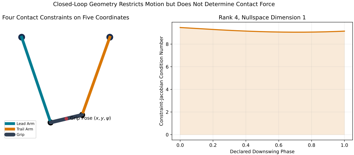
Figure 20.5: Closed-Loop Geometry Restricts Motion but Does Not Determine Contact Force
