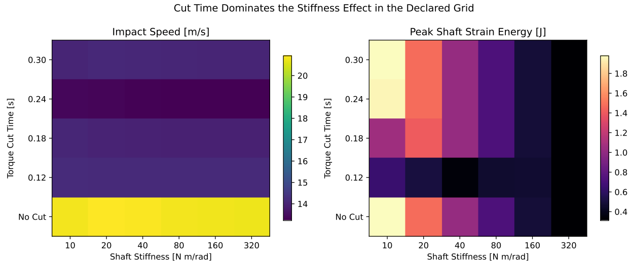
Figure 10.7: Torque-Cut Time Dominates the Stiffness Effect in the Declared Grid
