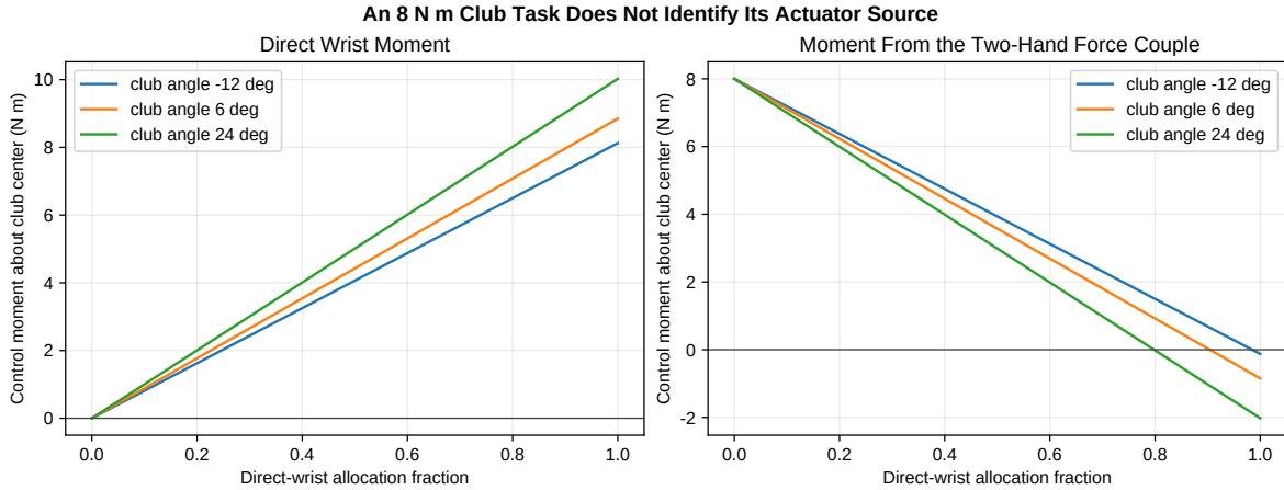
Figure 12.1: The Same Net Club-Moment Task Can Be Divided Between Direct Wrist Moment and a Two-Hand Force Couple
