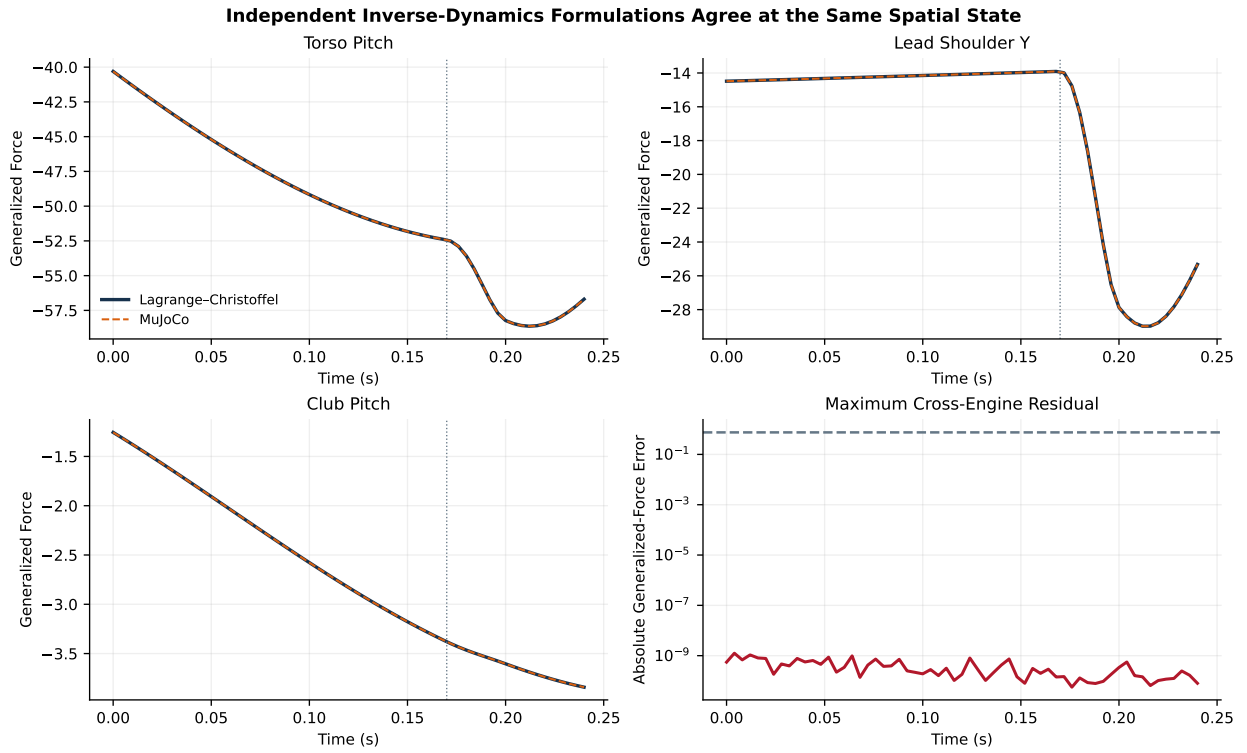
Figure 15.2: Independent Inverse-Dynamics Formulations Agree at the Same Spatial State
