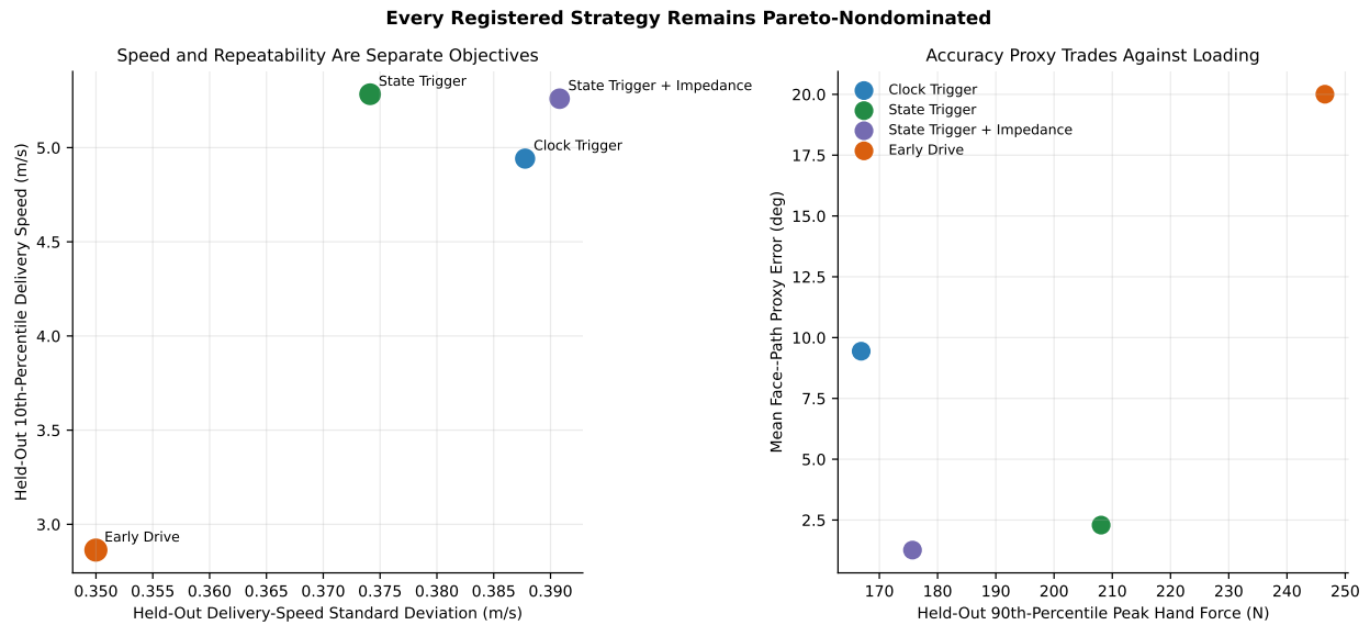
Figure 22.2: Held-out lower-tail speed and dispersion do not select the same program, and face/path error trades against peak hand force. Marker size in the left panel increases with peak-force exposure.
