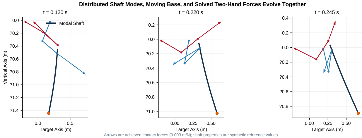
Figure 14.1: Forward Geometry, Distributed Shaft, and Achieved Grip Forces
