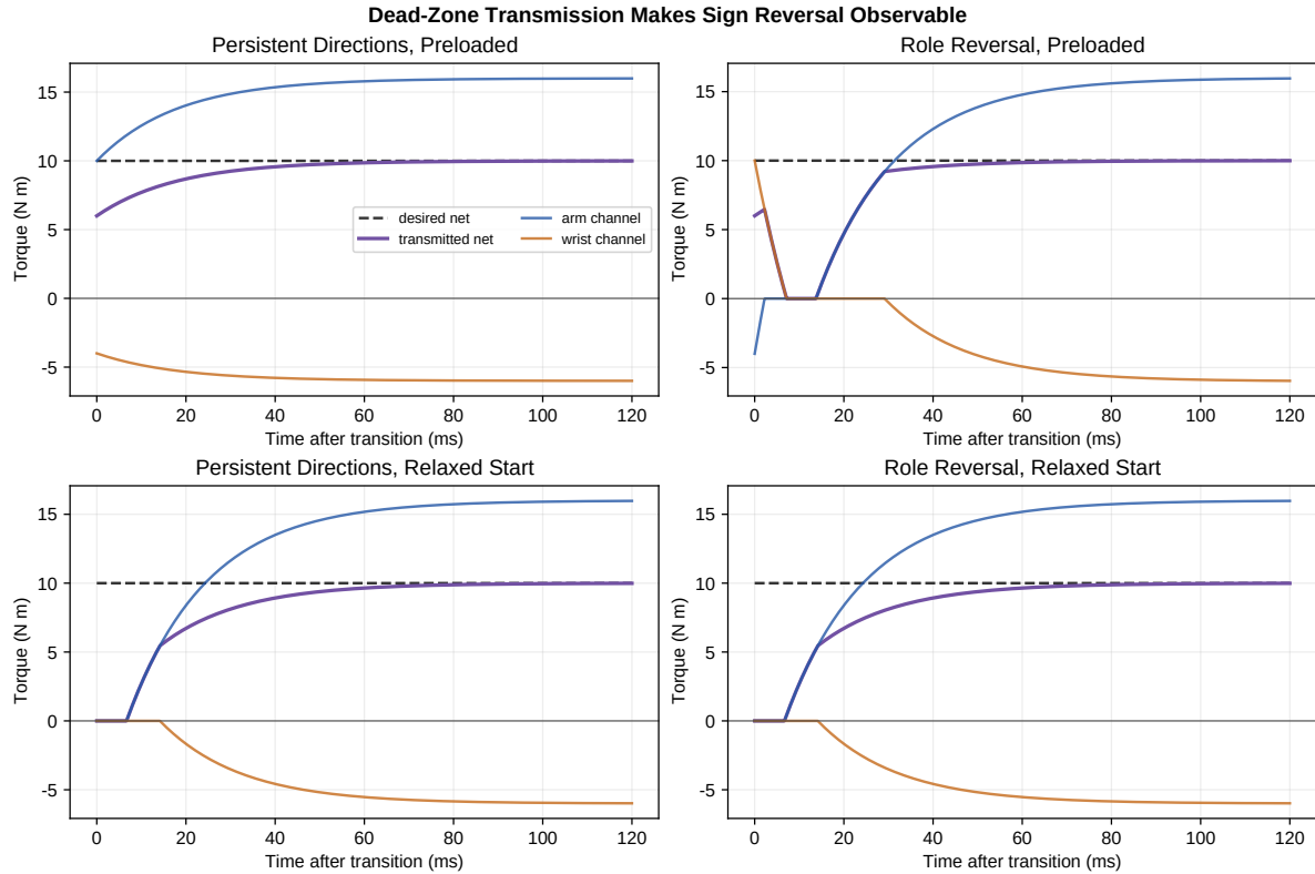
Figure 12.4: Transmission Continuity for Persistent-Direction and Role-Reversal Programs
