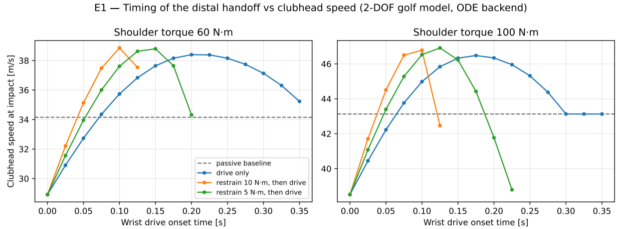
Figure 27.1: E1 sweep: clubhead speed at impact versus wrist-drive onset time, for drive-only and restrain-then-drive profiles at two shoulder-torque levels. Dashed line: fully passive wrist baseline.
