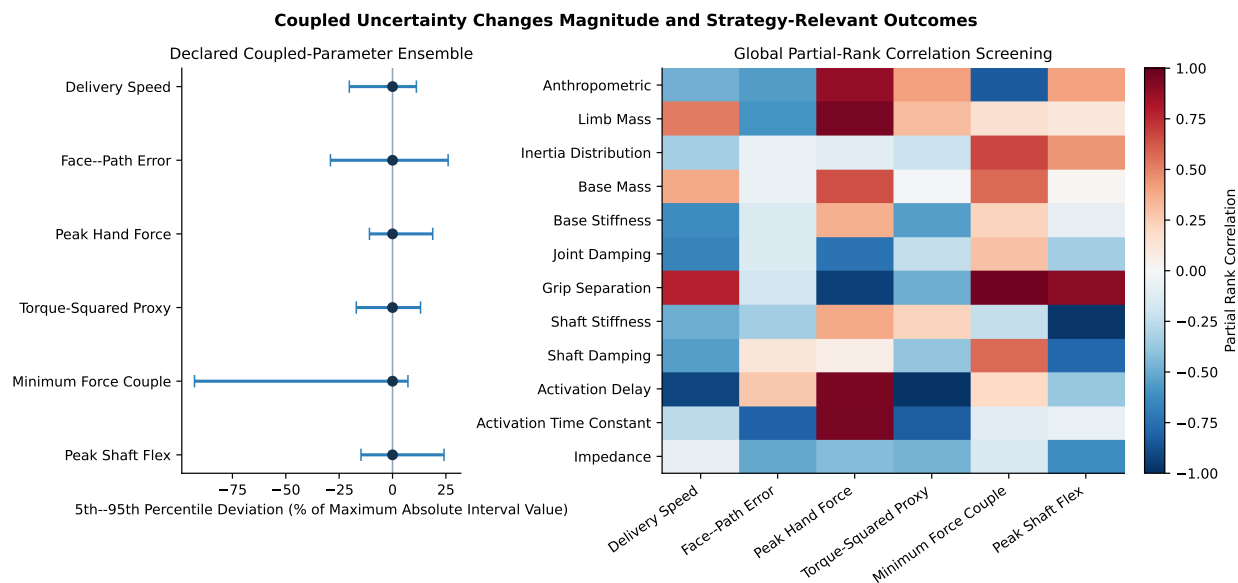
Figure 17.1: Uncertainty Intervals and PRCC Screening. Left: 5th-95th percentile ranges, normalized only for visual comparison. Right: partial rank correlations for the six registered outputs.
