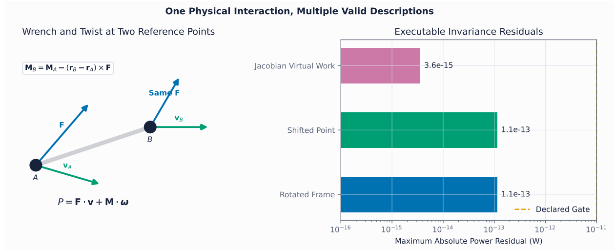
Figure 21.2: Power Is Invariant Under Consistent Frame and Reference-Point Changes
