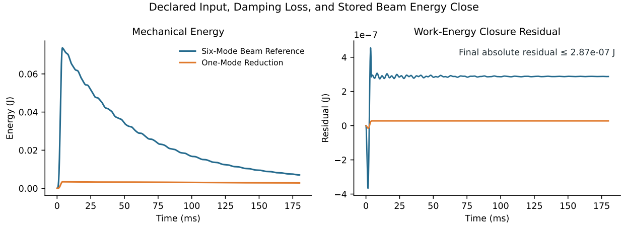
Figure 13.3: Beam Input, Damping, and Energy Closure
