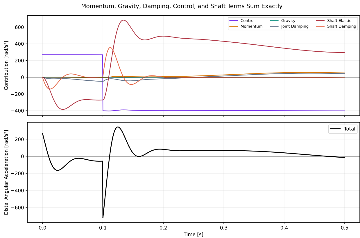
Figure 10.2: Momentum, Gravity, Damping, Control, and Shaft Terms Sum Exactly
