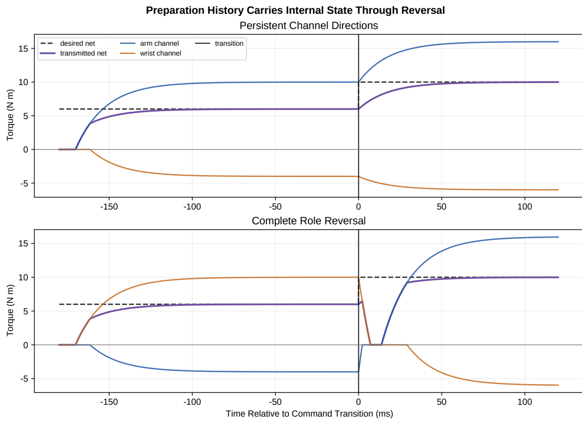
Figure 12.3: Continuous Preparation History and Command Transition
