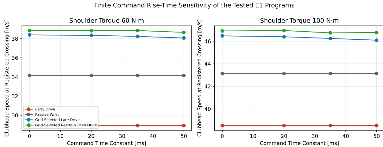
Figure 27.9: Finite Command Rise-Time Sensitivity of the Tested E1 Programs
