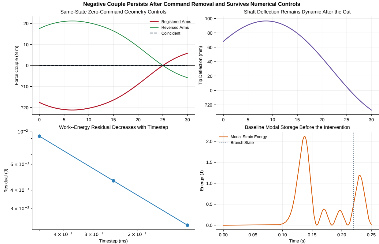
Figure 14.3: Same-State Killswitch, Geometry Controls, and Numerical Closure
