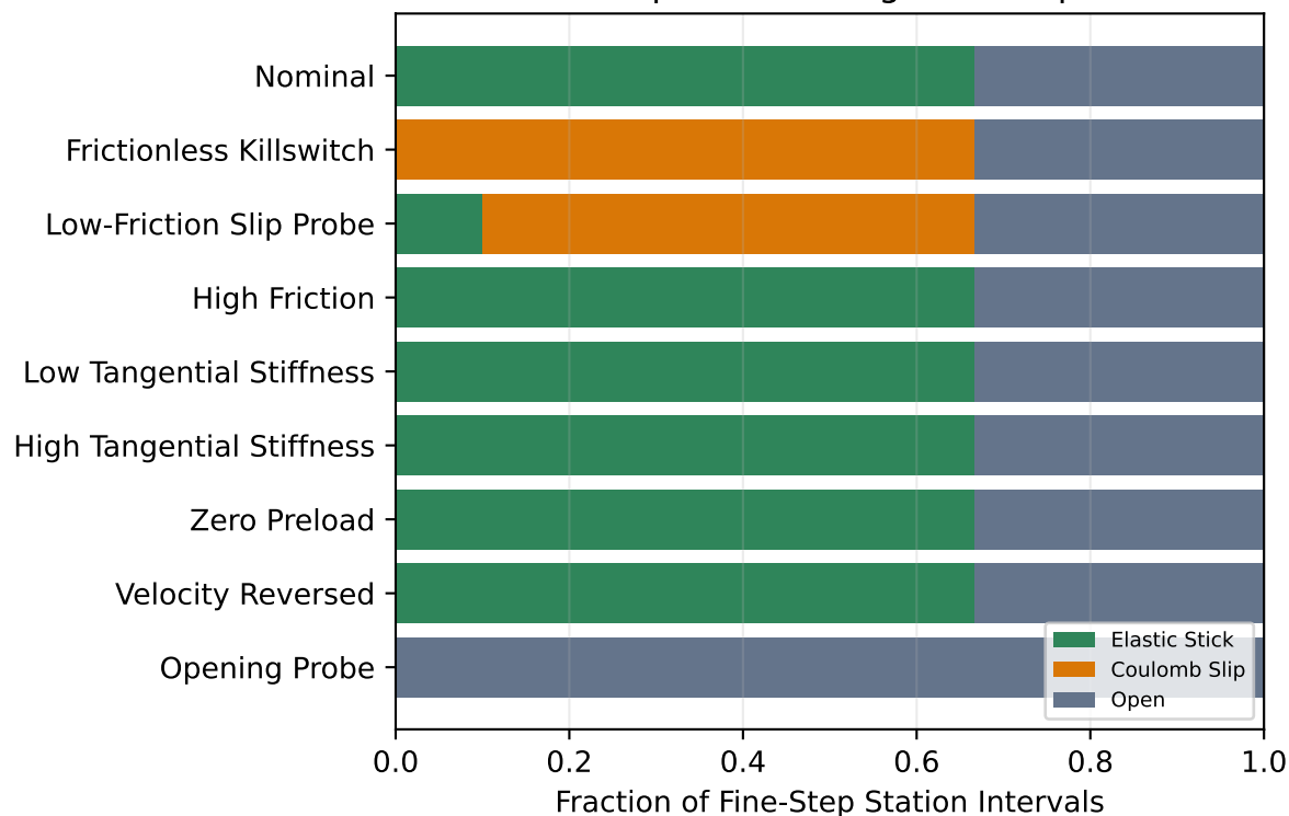
C. Fine-Step Contact-Regime Composition
