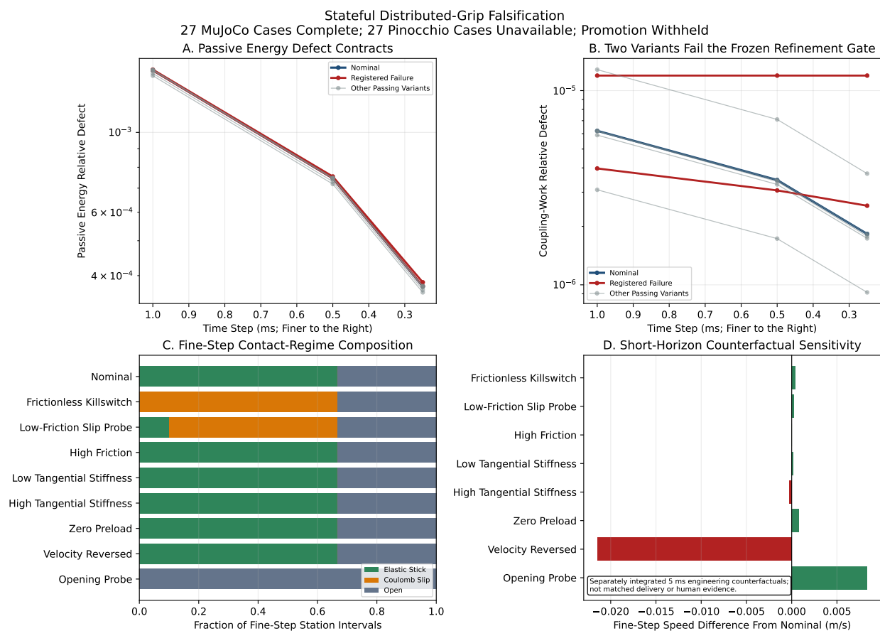
Figure 31.5: Stateful Distributed-Grip Falsification. Passive-energy defects contract in all nine MuJoCo variants, but the frictionless preload-release and low-friction slip cases fail the frozen coupling-work refinement criterion. Contact-regime counts and fine-step speed differences are short-horizon engineering-model diagnostics. Pinocchio was unavailable, so promotion and cross-engine parity are withheld.
