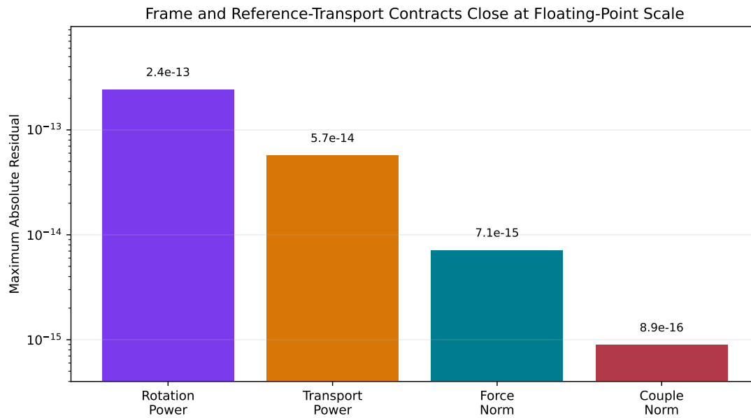
Figure 13.2: Frame and Reference-Transport Contracts Close at Floating-Point Scale
