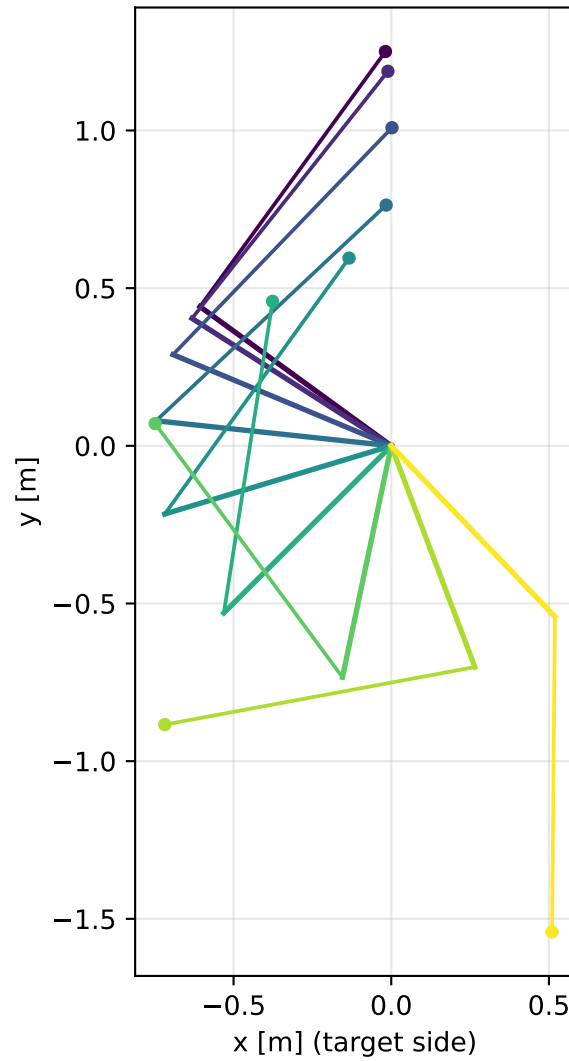
Figure 18.4: Stick-figure montage of the best restrain-then-drive swing in the swing plane (downswing progression at equal time steps).
