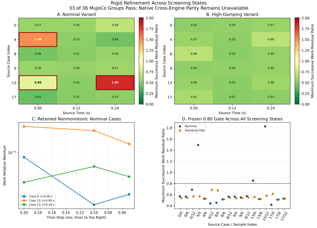
Figure 31.6: Rigid Refinement Across Screening States. The heatmaps and statewise scatter retain all three nominal refinement failures; the high-damping variant passes at every screened state. All individual closure tolerances pass, but nonmonotonic work-residual contraction and unavailable Pinocchio parity keep promotion false.
