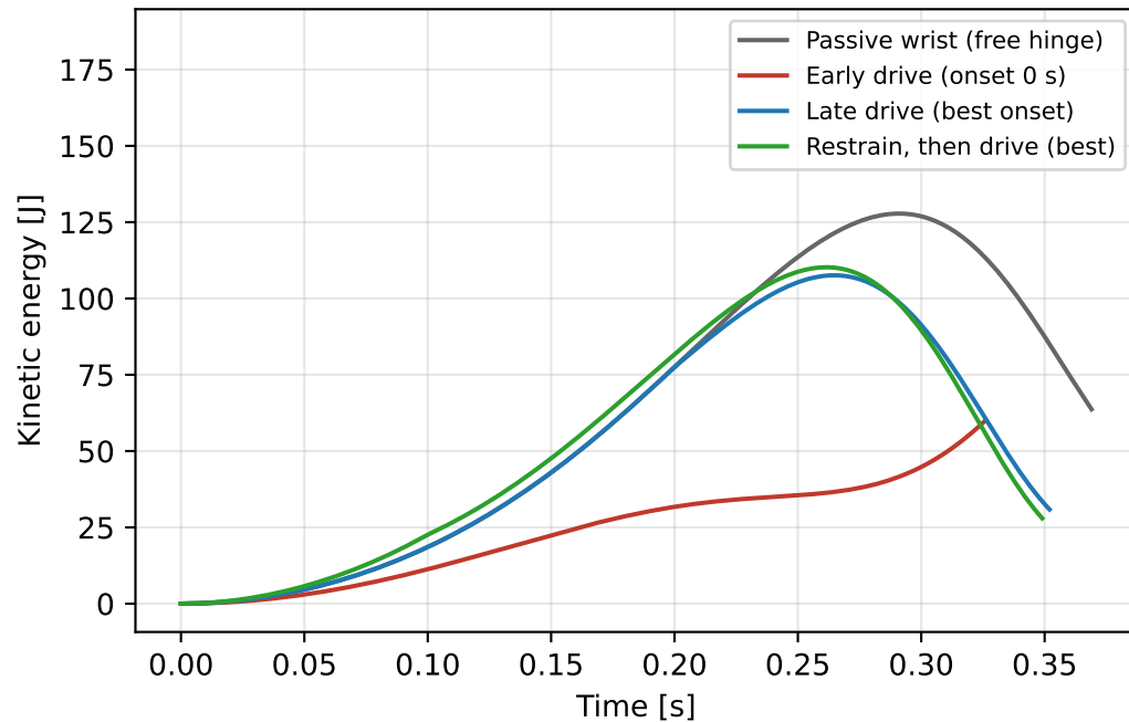
Arm segment kinetic energy
