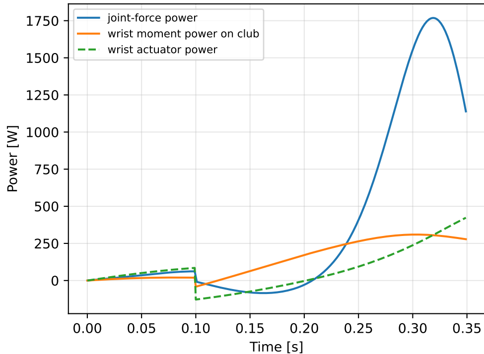
Interface powers — Restrain, then drive (best)
