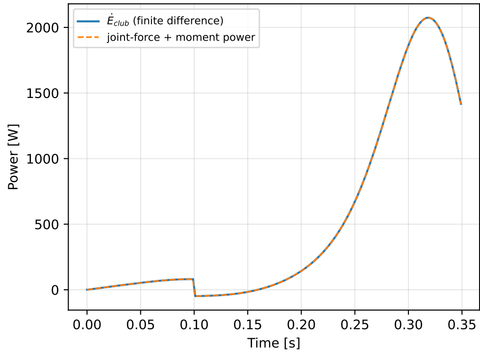
Segmental energy-balance check (Robertson-Winter)
