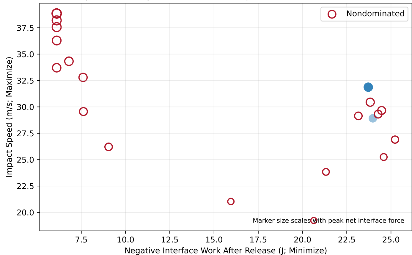
Speed, Braking, and Peak-Force Objectives Remain in Tension
