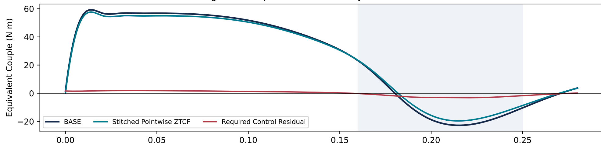
Drift-Aware Preview Improves a Delayed Actuator's Couple Tracking
