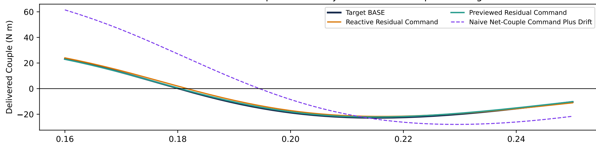
The Best Preview Depends on the Assumed Actuator Time Constant
