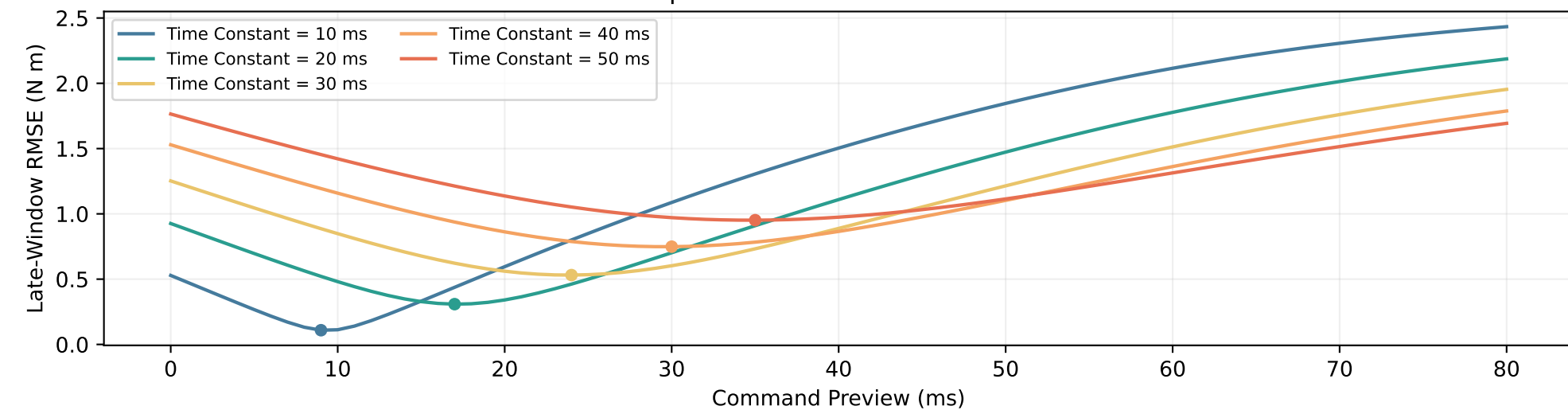
The Best Preview Depends on the Assumed Actuator Time Constant
