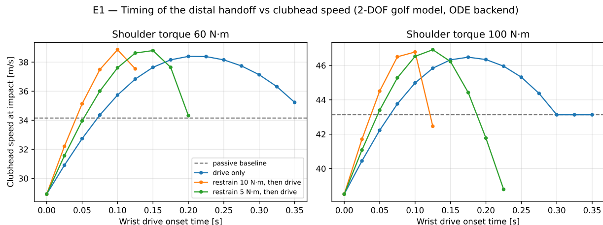
Figure 17.1: E1 sweep: clubhead speed at impact versus wrist-drive onset time, for drive-only and restrain-then-drive profiles at two shoulder-torque levels. Dashed line: fully passive wrist baseline.
