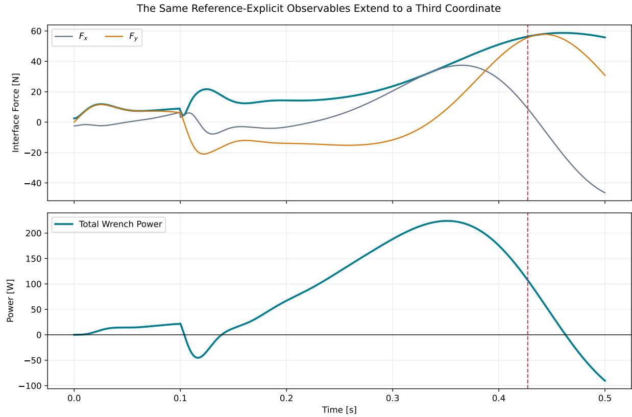
Figure 12.3: The Same Reference-Explicit Observables Extend to a Third Coordinate
