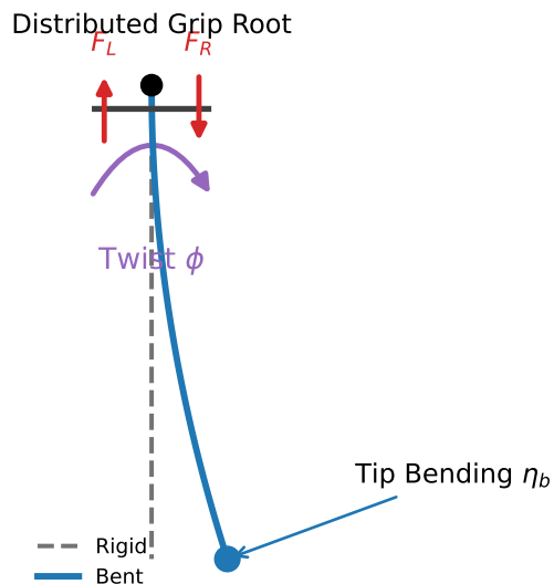
A. Passive Shaft Coordinates and Grip Wrench
