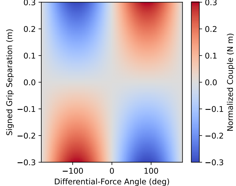
Bilateral Force-Couple Geometry
