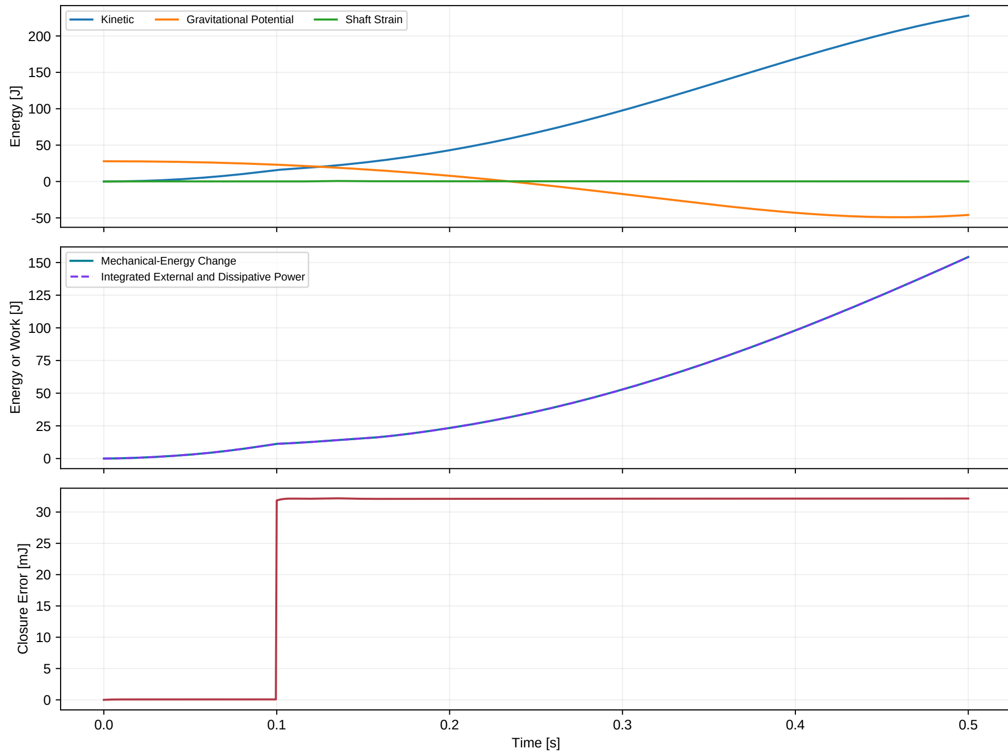
Shaft Strain Energy Is Small but Explicitly Closed
