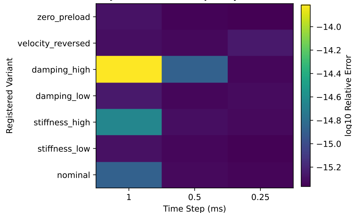
MuJoCo--Pinocchio Trajectory Difference
