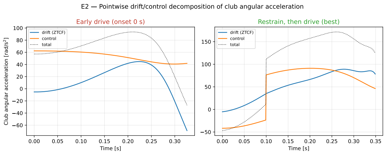
Figure 20.8: Pointwise drift (ZTCF) versus control decomposition of club absolute angular acceleration, for the early-drive (left) and best restrain-then-drive (right) programs.
