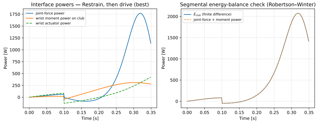
Figure 20.7: Left: wrist-interface powers for the best restrain-then-drive swing. Right: segmental energy-balance check — club mechanical-energy rate versus the sum of interface powers.
