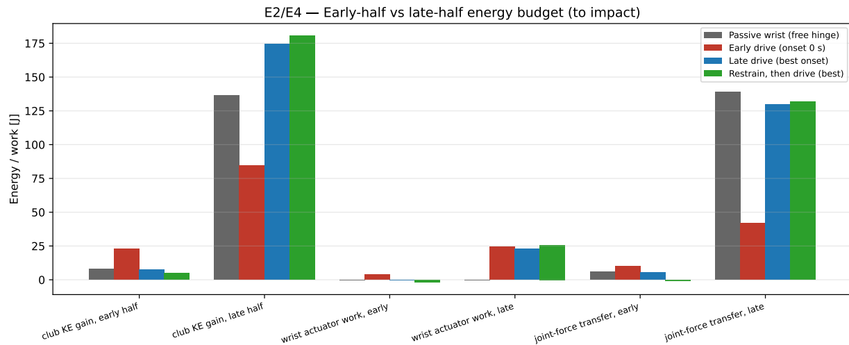
Figure 20.6: Early-half versus late-half energy budget (club kinetic-energy gain, wrist actuator work, integrated joint-force transfer) for the representative programs.
