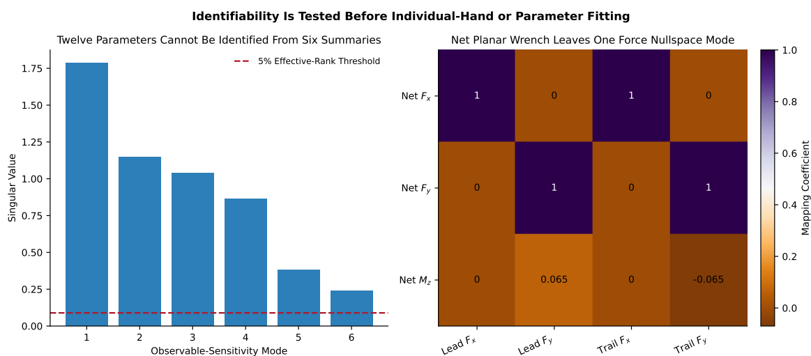
Figure 12.2: Identifiability Audit. The net planar wrench cannot uniquely allocate both hand forces, and six summary observables cannot identify the full 12-parameter vector.
