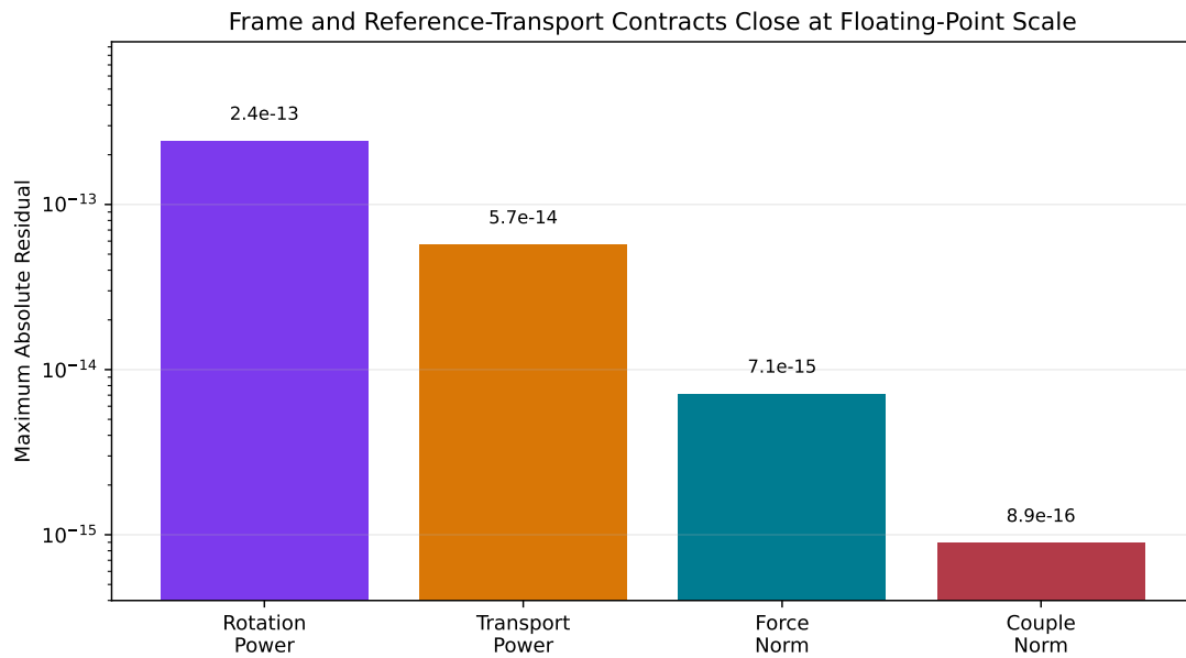
Figure 15.2: Frame and Reference-Transport Contracts Close at Floating-Point Scale
