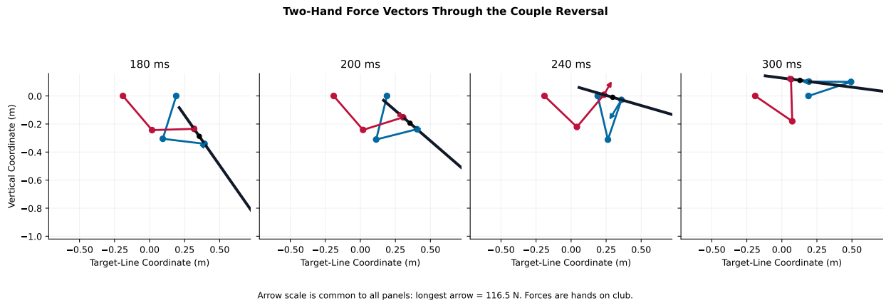
Figure 7.2: Two-Hand Force Vectors Through the Couple Reversal. Blue and red arrows are the right- and left-hand forces on the club; all panels use the same force scale. Black denotes the floating club, colored links denote the two arms, and the black point is the declared club center.
