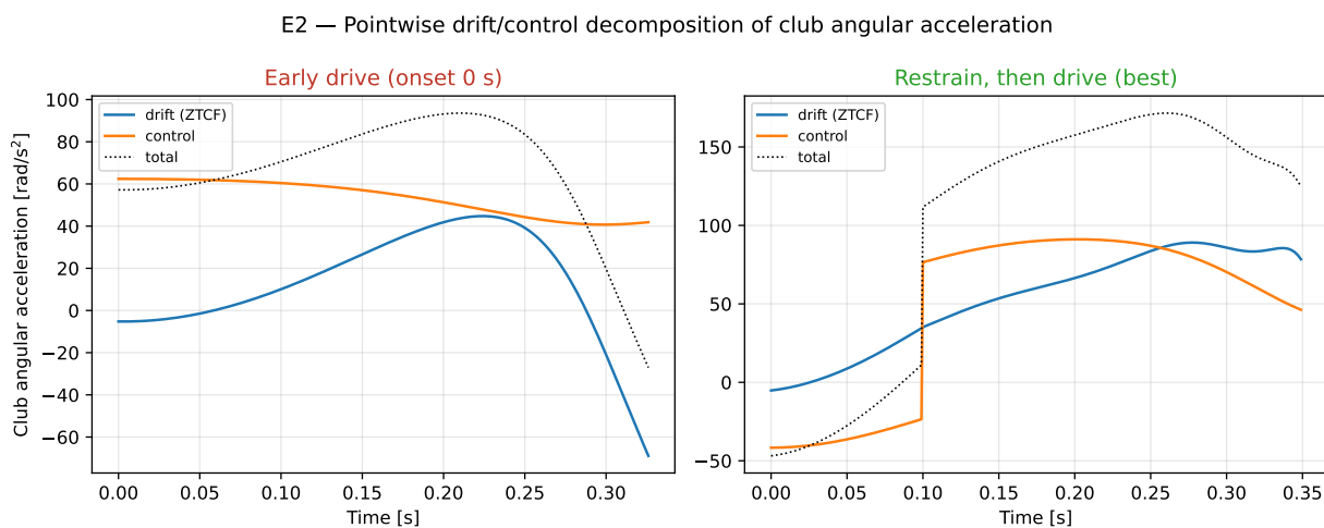
Figure 14.8: Pointwise drift (ZTCF) versus control decomposition of club absolute angular acceleration, for the early-drive (left) and best restrain-then-drive (right) programs.
