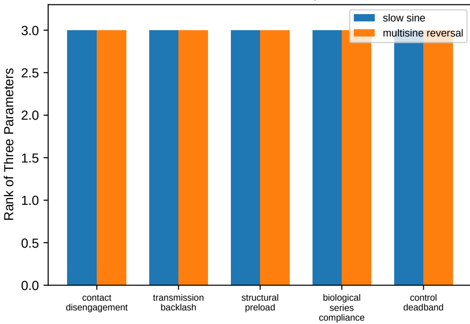
Local Scaled Sensitivity Rank
