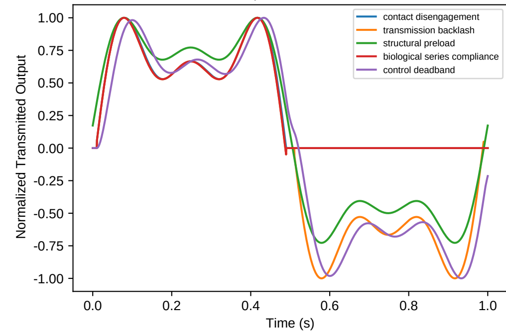
Normalized Outputs Are Not Class Labels
