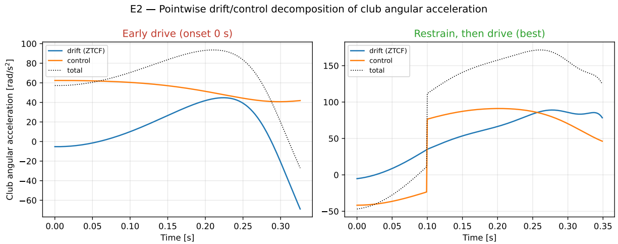
Figure 28.8: Pointwise drift (ZTCF) versus control decomposition of club absolute angular acceleration, for the early-drive (left) and best restrain-then-drive (right) programs.
