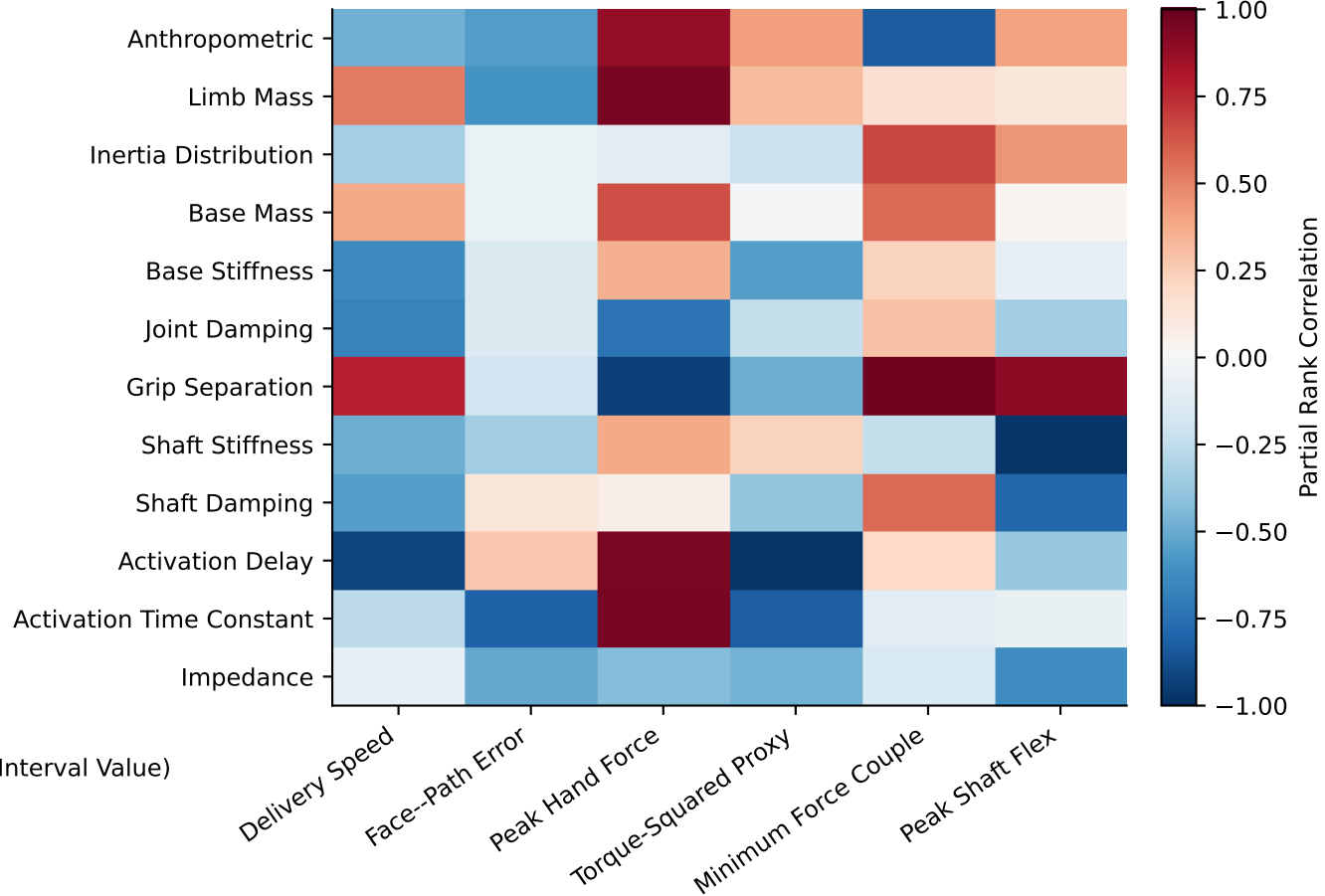
Global Partial-Rank Correlation Screening
