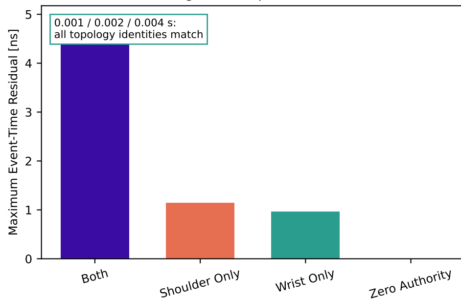
Integration-Step Refinement
