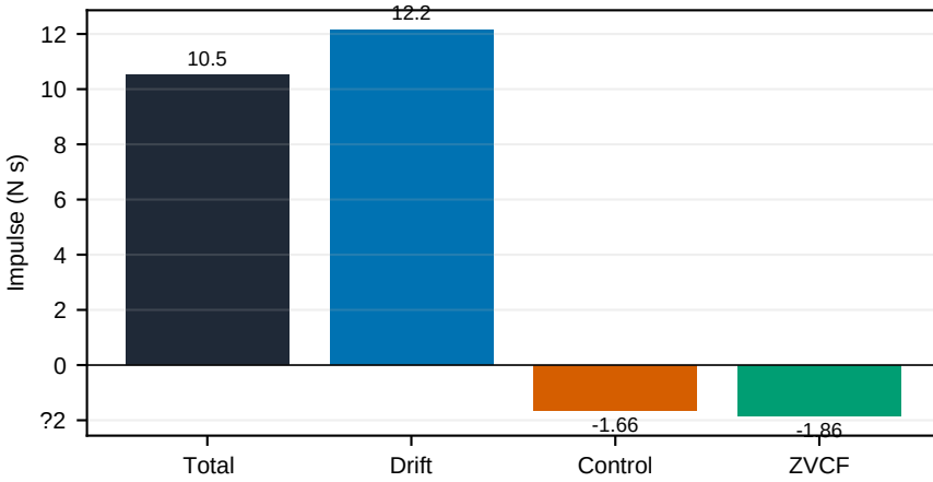
One-Arm Three-Link: Target-Direction Vector Impulse
