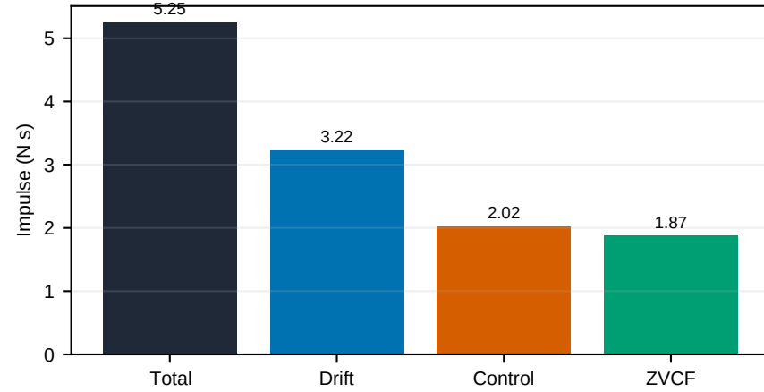
Two-Arm Closed Loop: Target-Direction Vector Impulse
