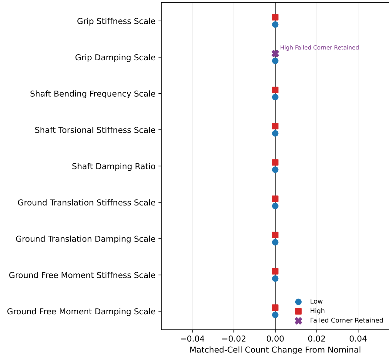
Ground Screen: Nominal 0/384 Matched Cells
