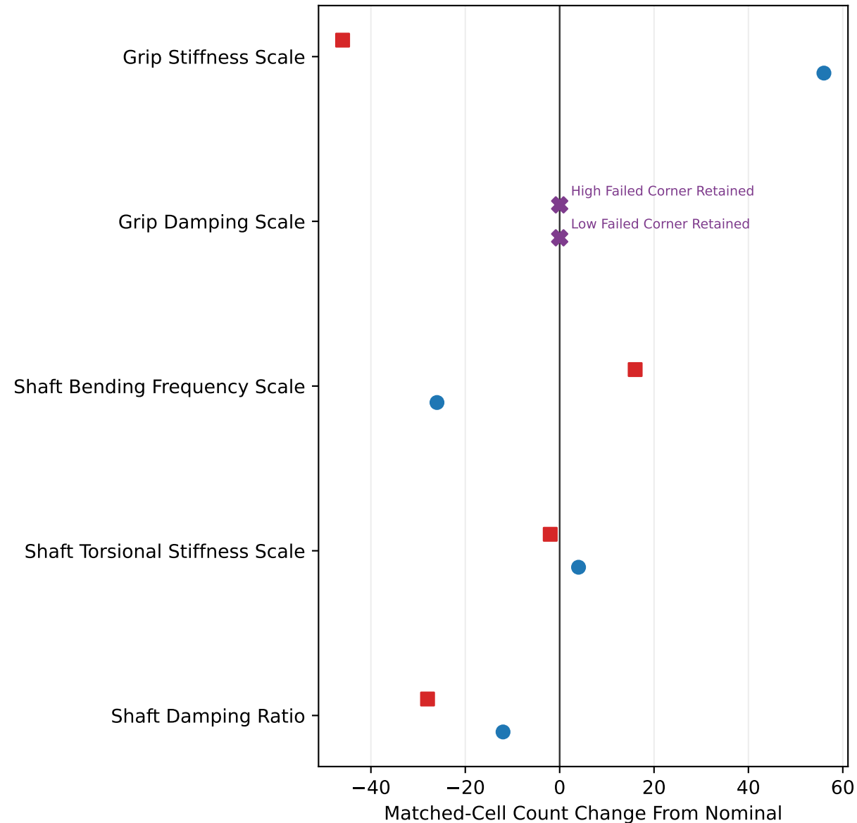
Shaft Screen: Nominal 126/384 Matched Cells
