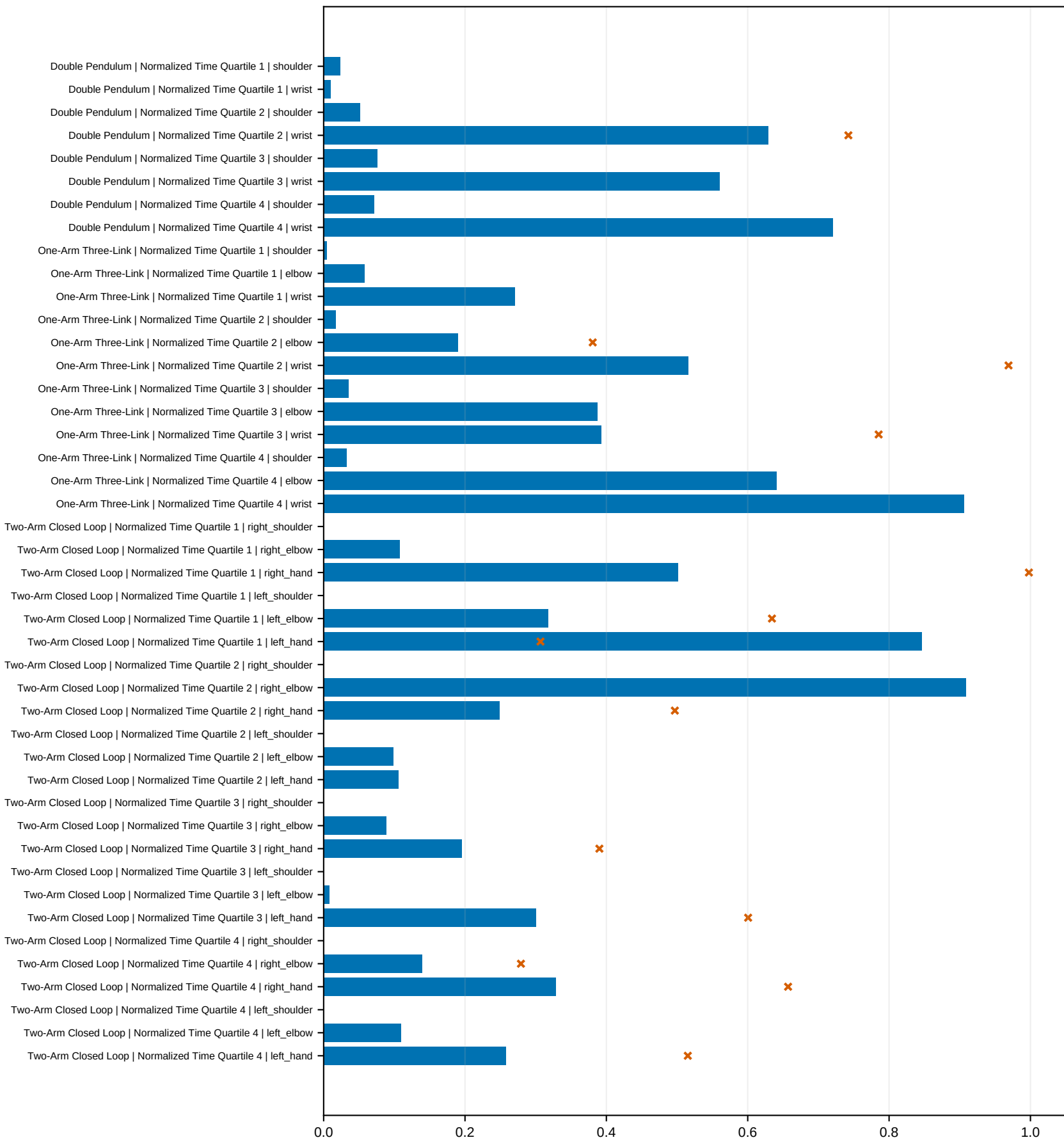
Phase-Resolved Drift Shares and Cancellation
