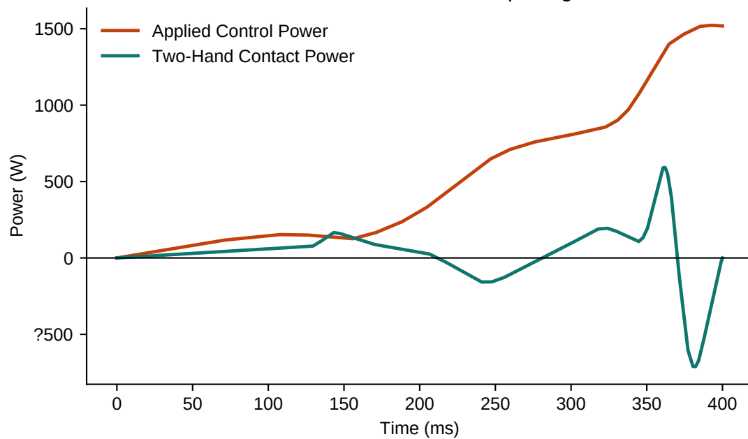
Power Is Distinct from Couple Sign
