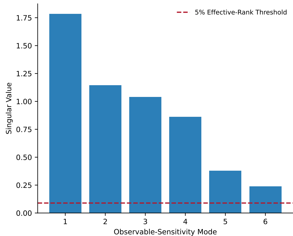
Twelve Parameters Cannot Be Identified From Six Summaries
