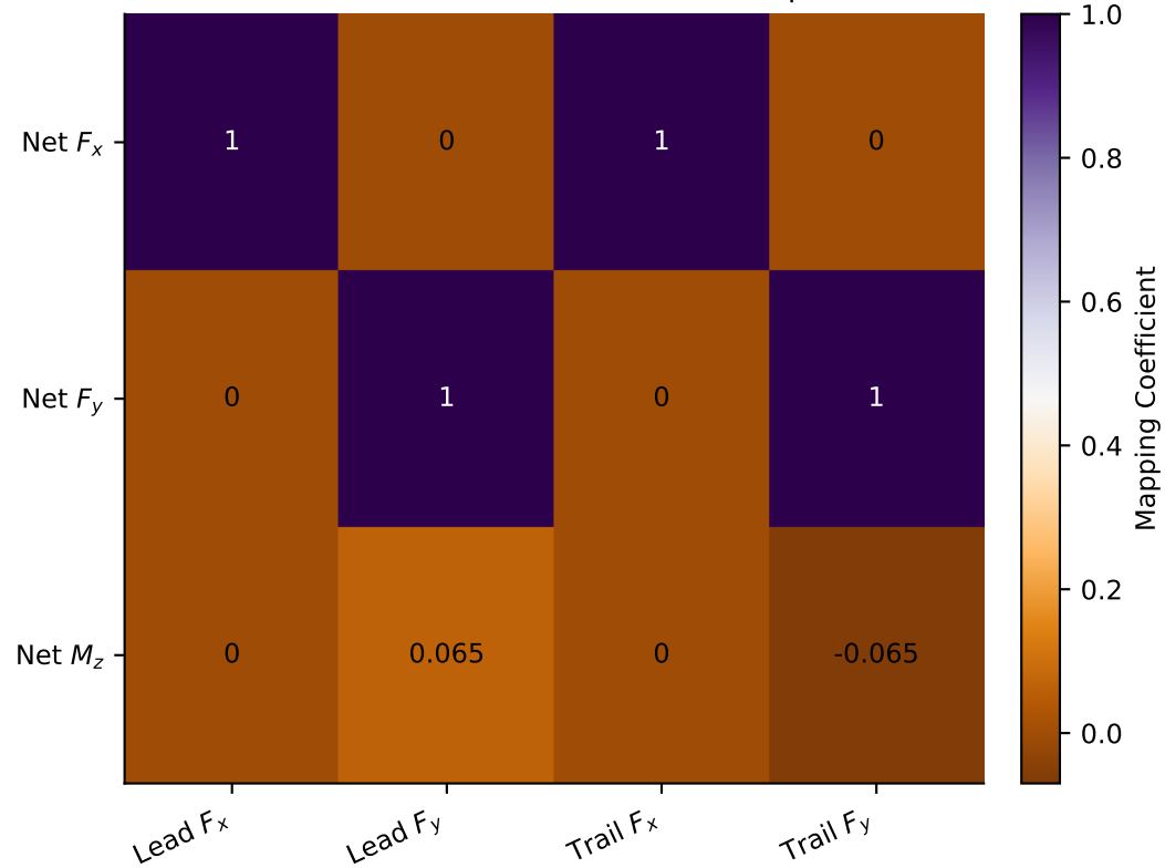
Net Planar Wrench Leaves One Force Nullspace Mode
