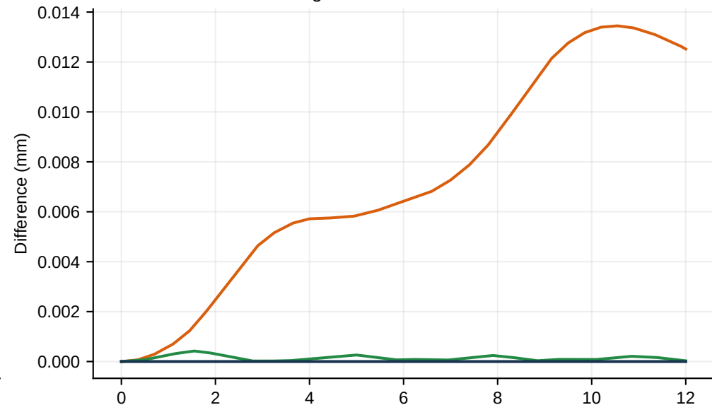
Resolved 2 ms Wrist-Moment Pulse: Position Error vs Six Modes
