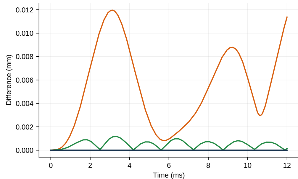
Resolved 2 ms Wrist-Moment Pulse: Position Error vs Six Modes
