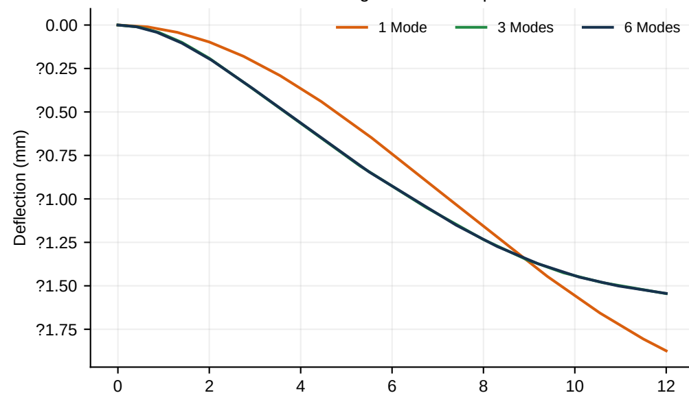
Resolved 2 ms Wrist-Moment Pulse: Tip Deflection
