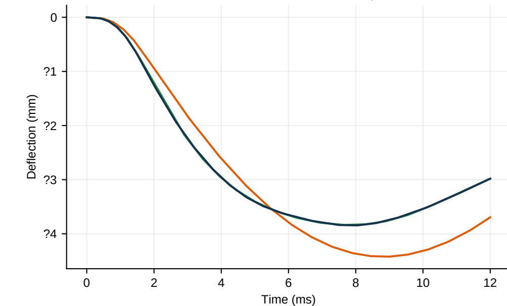
Resolved 2 ms Wrist-Moment Pulse: Tip Deflection
