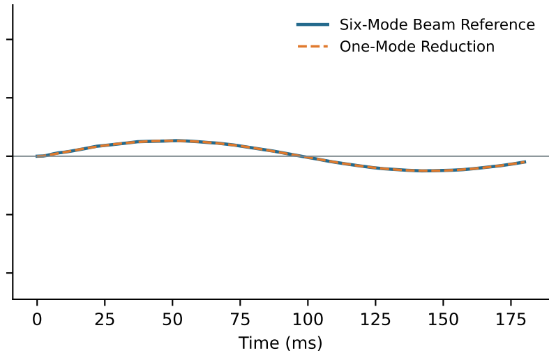
Short Tip-Force and Moment Pulse
