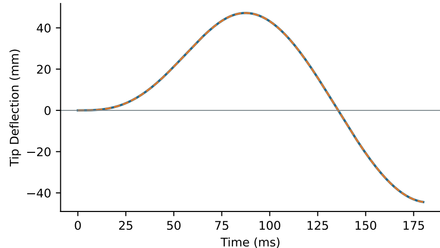
Slow Tip-Force Pulse
