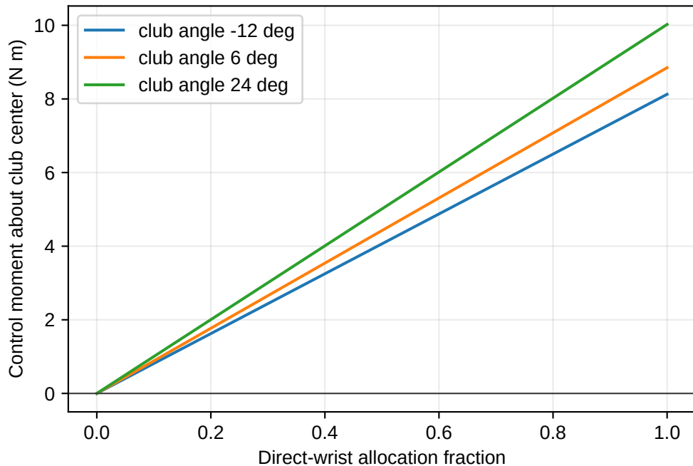
Direct Wrist Moment
