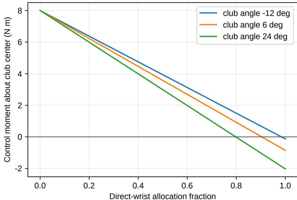
Moment From the Two-Hand Force Couple
