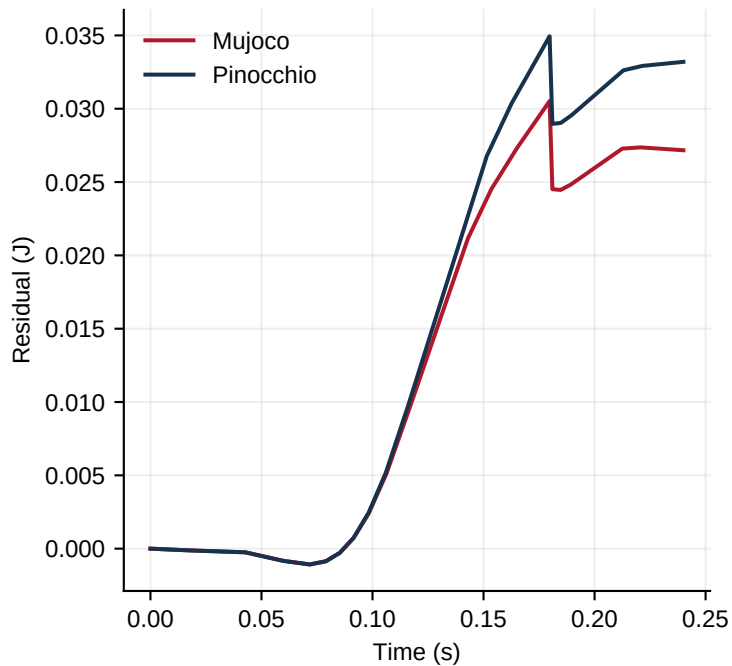
Work–Energy Residual
