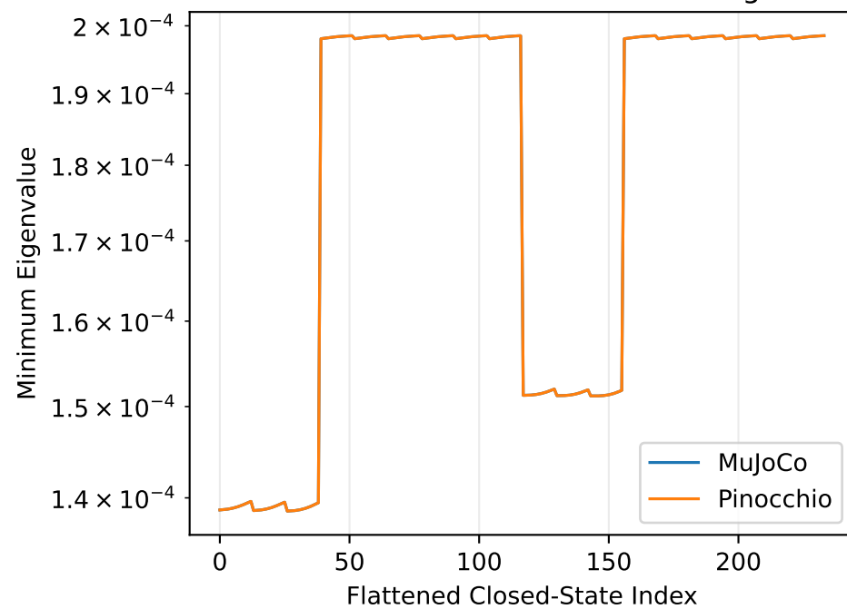
Positive-Definite Mass-Matrix Margin
