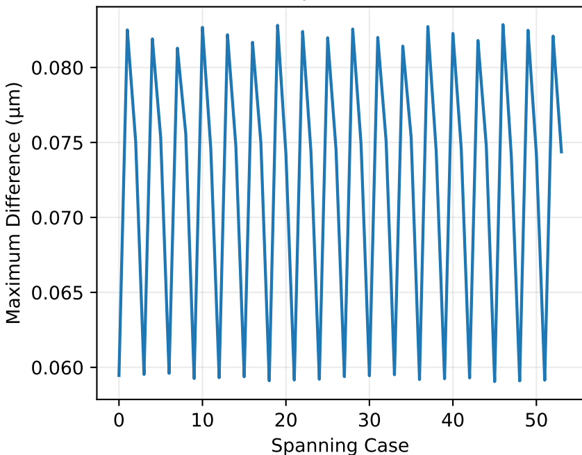
Inertia-and-Bias Transport Club-Position Difference
