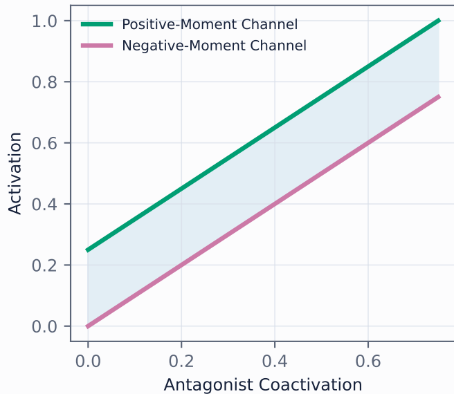
Activation Family
