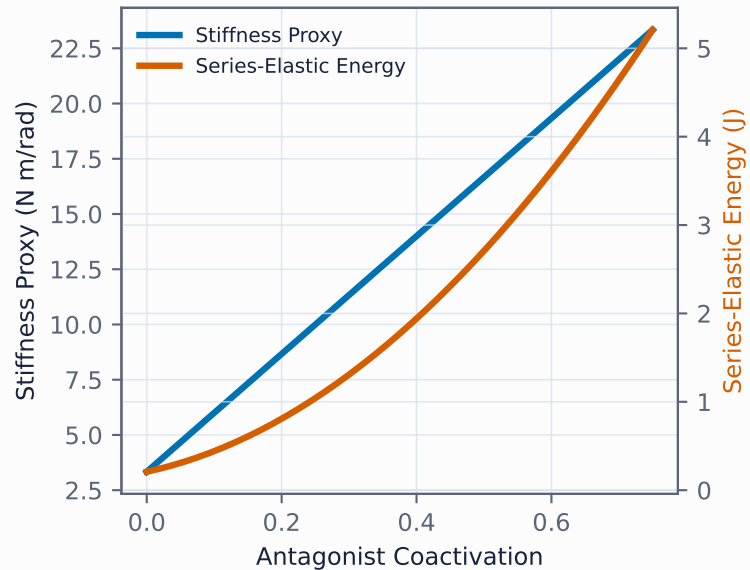
Internal Consequences
