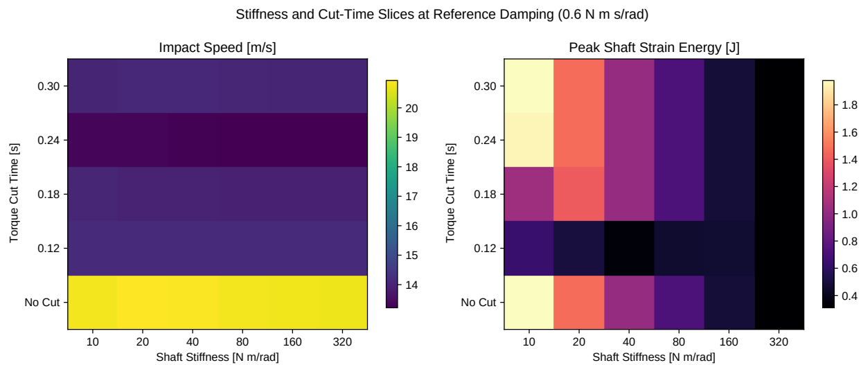
Figure 12.7: Stiffness and Torque-Cut-Time Slices at Reference Damping
