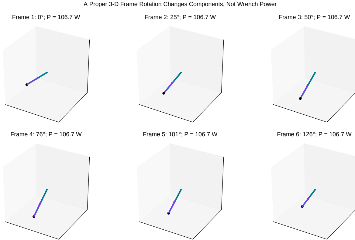
Figure 22.7: A Proper 3-D Frame Rotation Changes Components, Not Wrench Power
