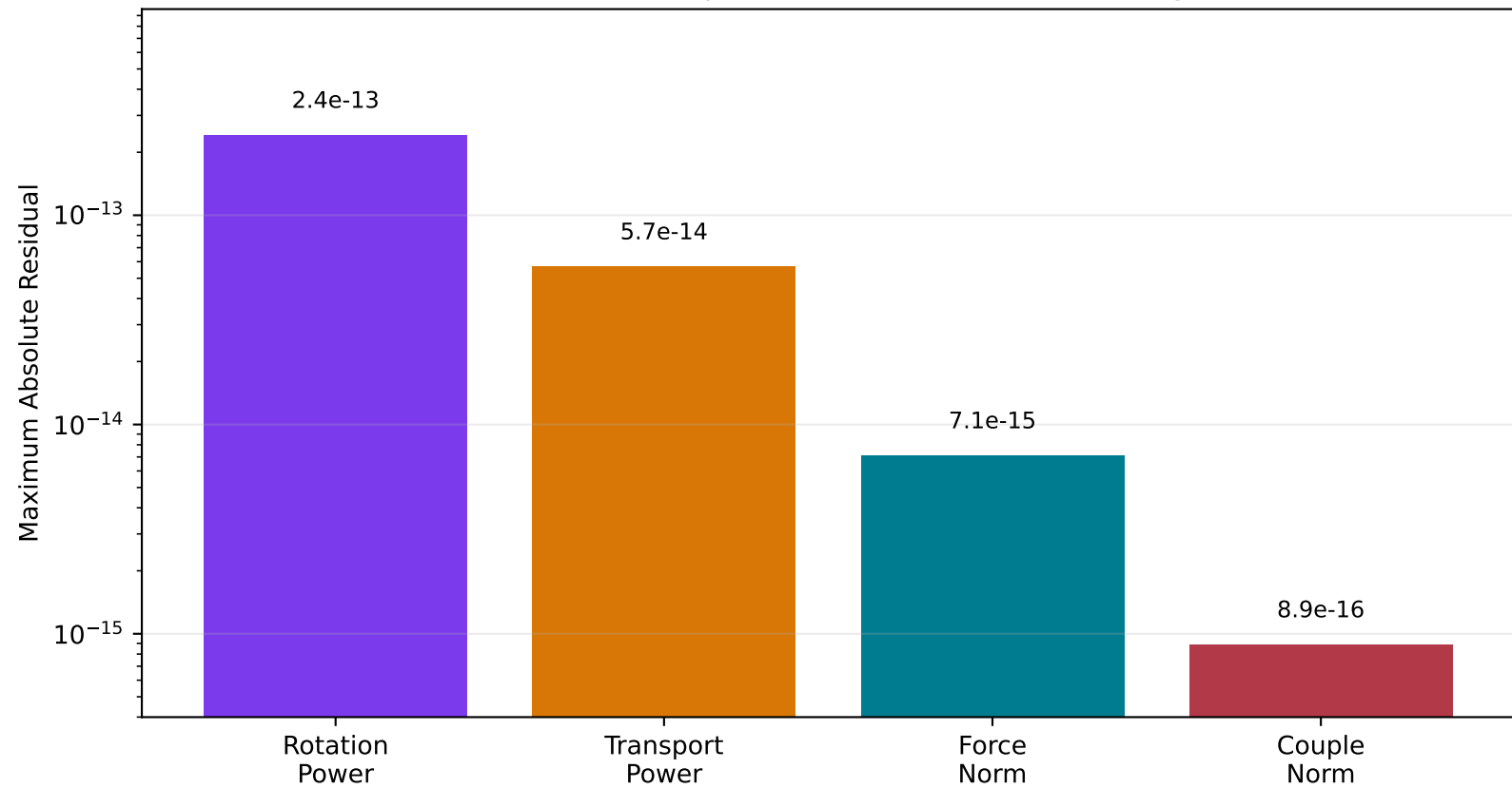
Frame and Reference-Transport Contracts Close at Floating-Point Scale
