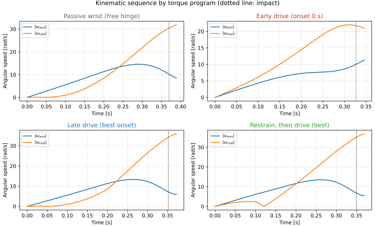
Figure 16.3: Kinematic sequence (arm and club angular speeds) for the four representative programs at \tau_s = 60 \text{ N} \cdot \text{m} . Dotted vertical line: impact.
