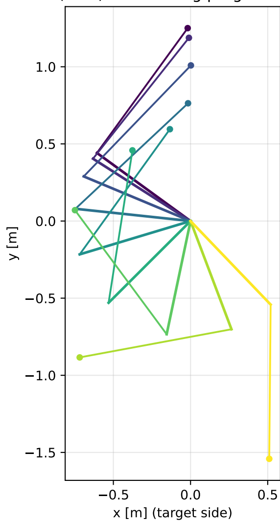
Figure 16.4: Stick-figure montage of the best restrain-then-drive swing in the swing plane (downswing progression at equal time steps).
