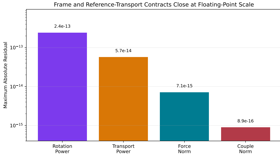
Figure 11.2: Frame and Reference-Transport Contracts Close at Floating-Point Scale
