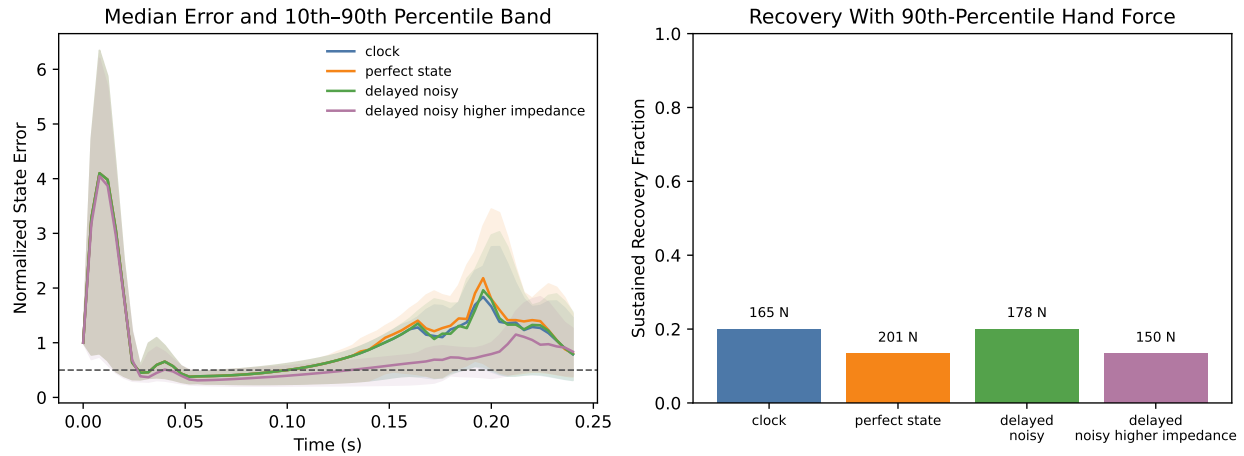
Figure 30.1: Trajectory-Level Recovery Under Matched Initial-State Perturbations. Bands show the held-out engineering envelope; labels above the recovery bars give 90th-percentile individual-hand force.
