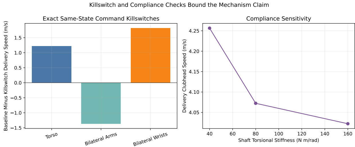
Figure 6.10: Delivery-speed changes under exact same-state command killswitches and shaft-stiffness sensitivity. A positive bar means the continued baseline command finishes faster than the corresponding command-zero branch.
