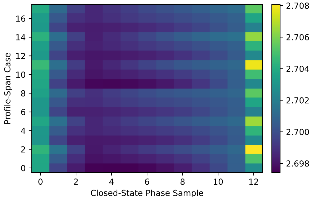
Zero-Preload Closure Leakage
