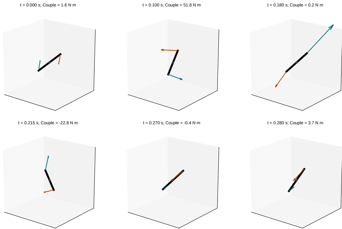
Figure 8.6: Three-Dimensional View of the Archived Two-Hand Force System
