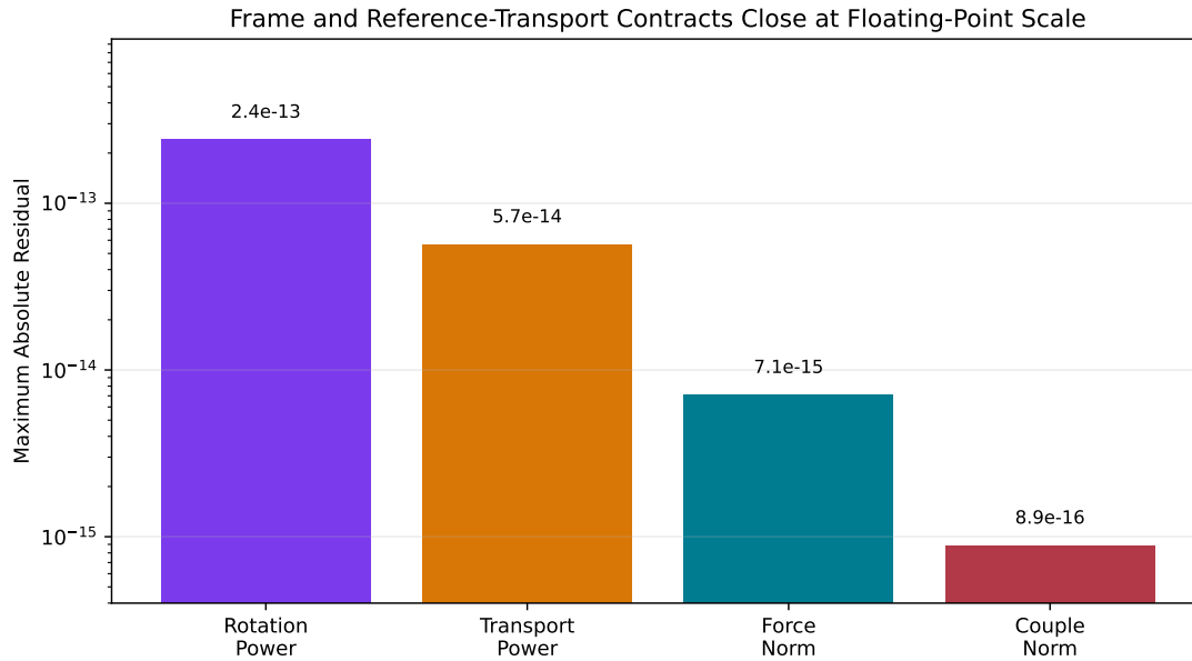
Figure 10.2: Frame and Reference-Transport Contracts Close at Floating-Point Scale
