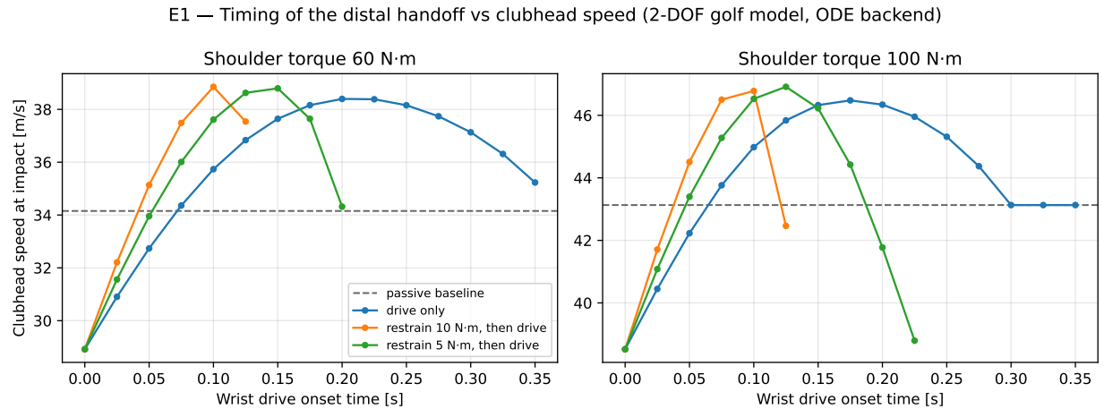
Figure 15.1: E1 sweep: clubhead speed at impact versus wrist-drive onset time, for drive-only and restrain-then-drive profiles at two shoulder-torque levels. Dashed line: fully passive wrist baseline.
