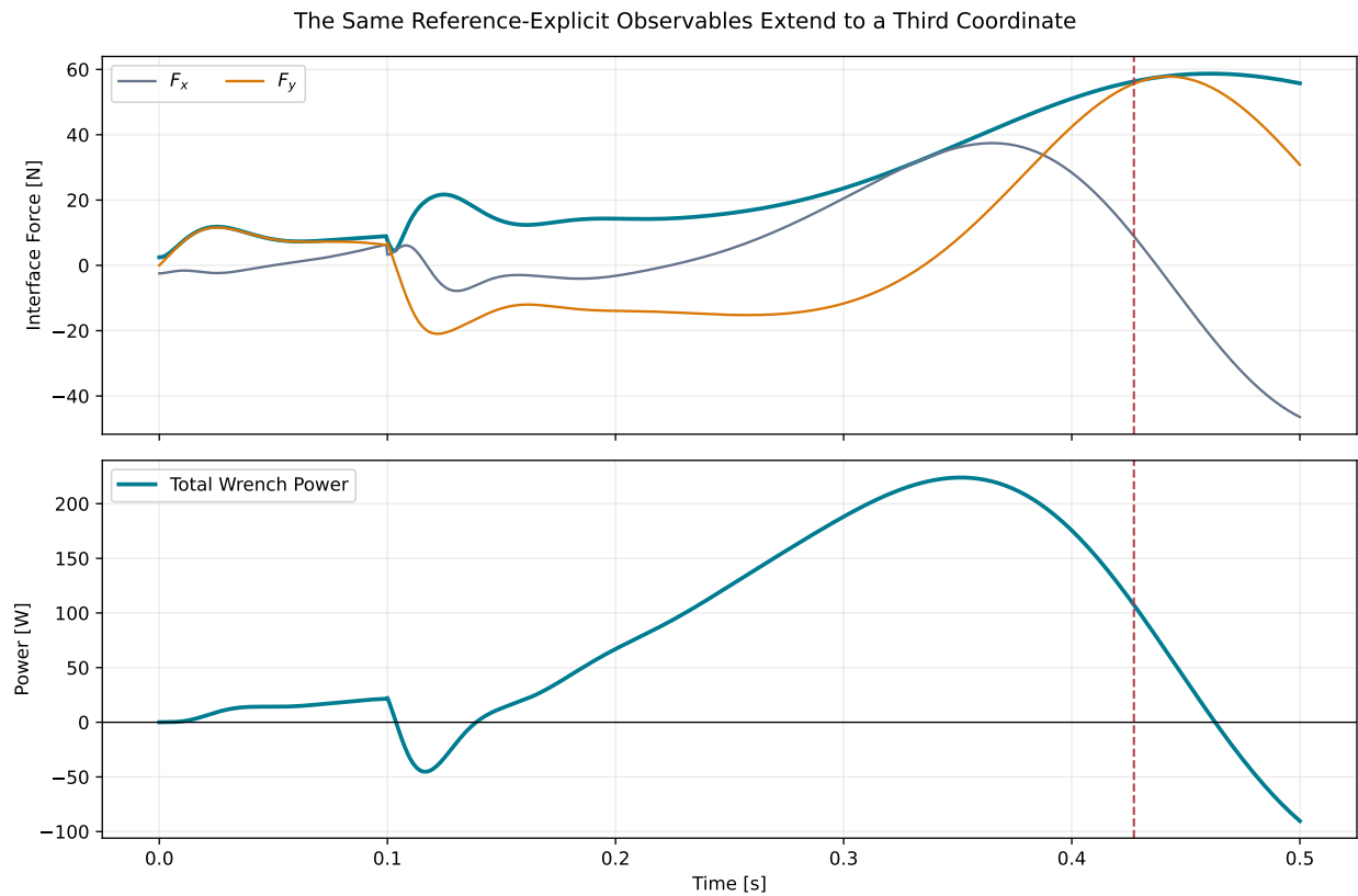
Figure 10.3: The Same Reference-Explicit Observables Extend to a Third Coordinate
