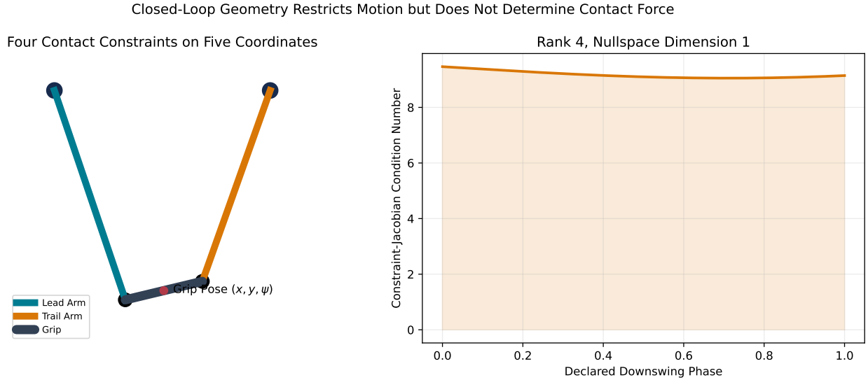
Figure 10.5: Closed-Loop Geometry Restricts Motion but Does Not Determine Contact Force
