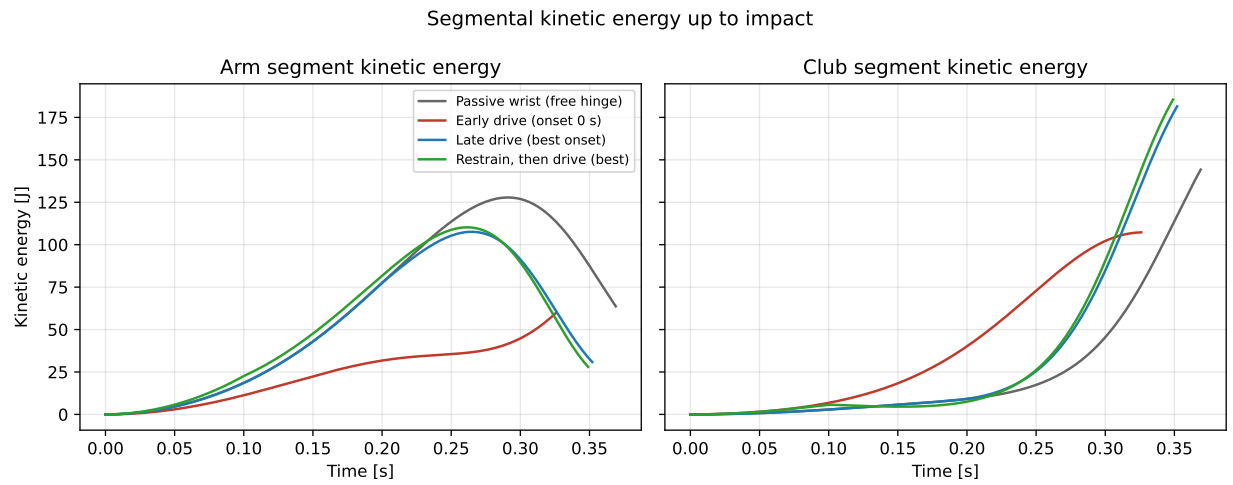
Figure 15.5: Segmental kinetic energies up to impact for the four representative programs.
