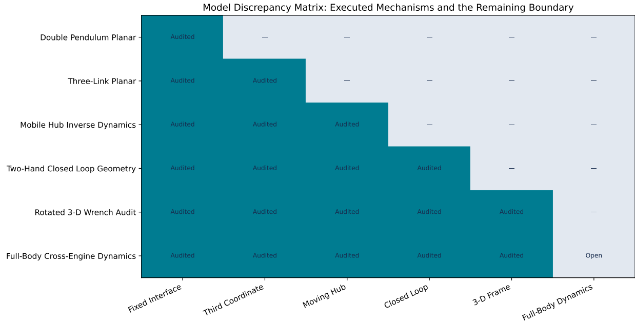
Figure 10.7: Model Discrepancy Matrix: Executed Mechanisms and the Remaining Boundary
