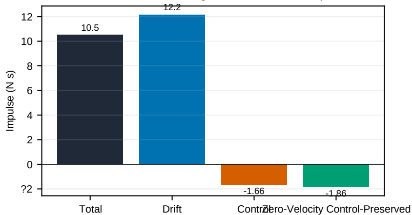
One-Arm Three-Link: Target-Direction Vector Impulse
