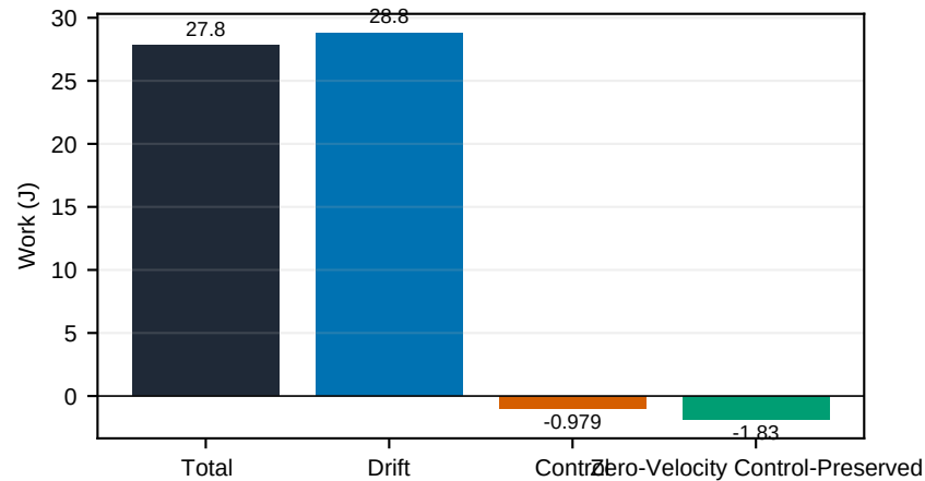
Two-Arm Closed Loop: Force Work
