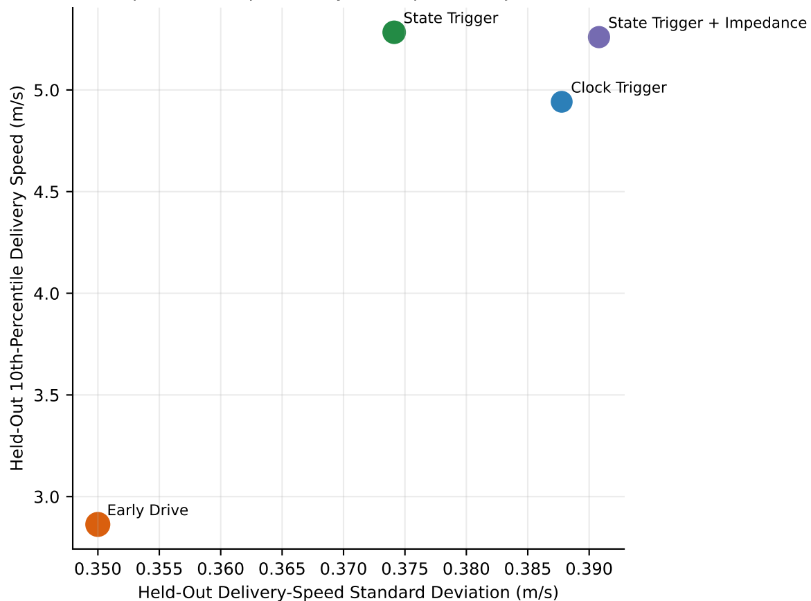
Speed and Repeatability Are Separate Objectives
