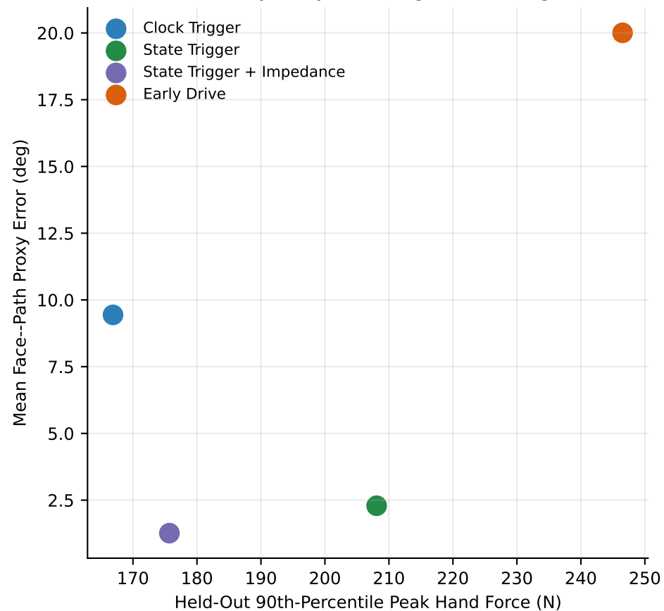
Accuracy Proxy Trades Against Loading
