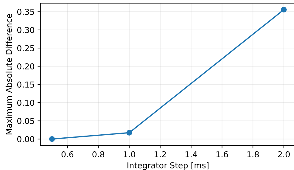
Force-Work Difference [J]
