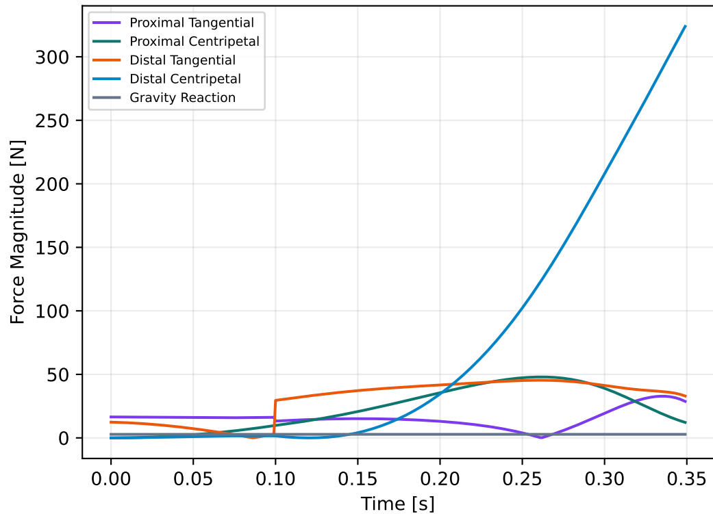
Exact Inertial Component Magnitudes
