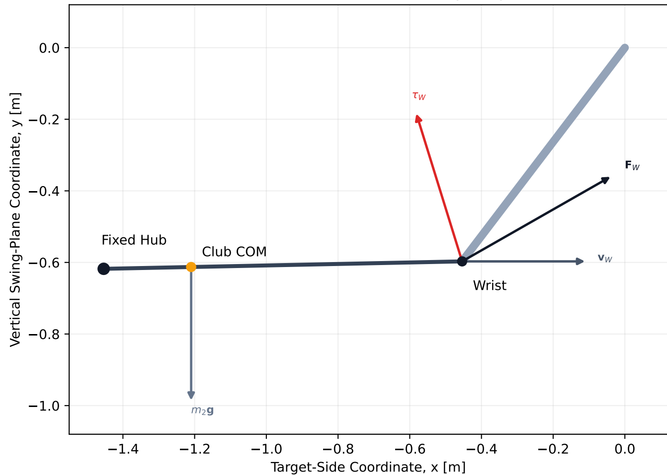
Double-Pendulum Club Free-Body Diagram
